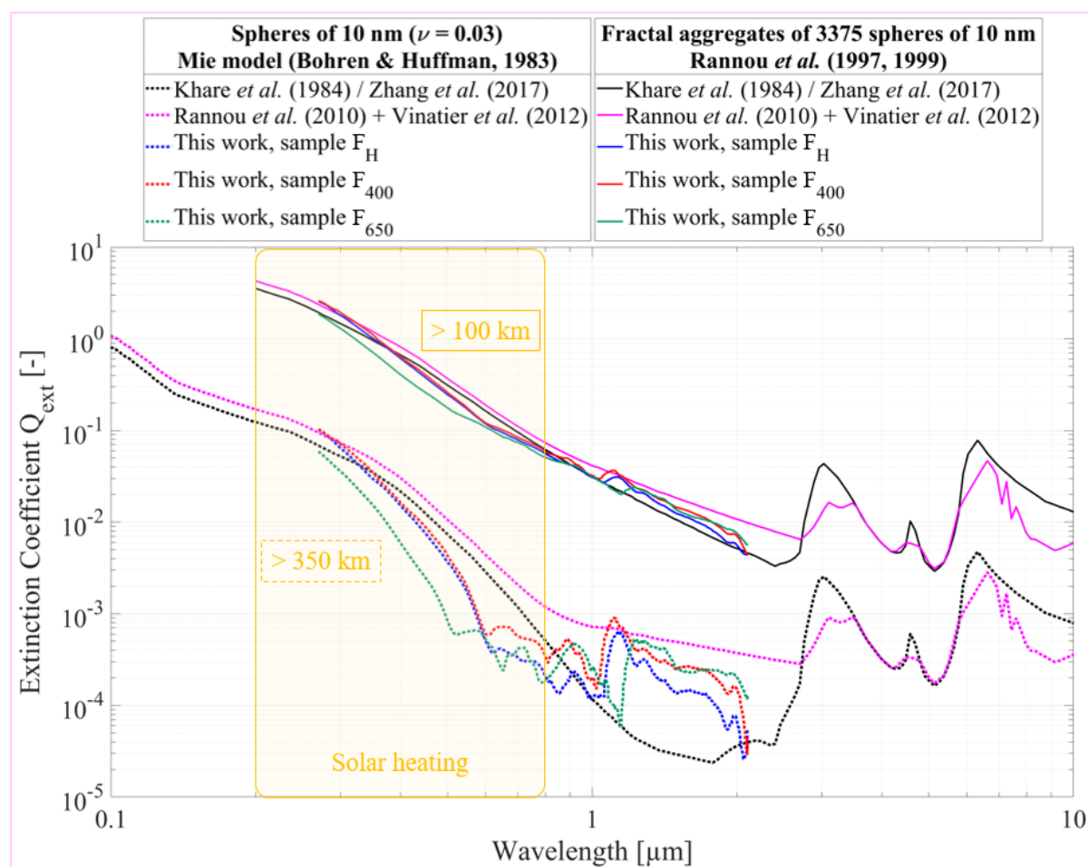
Figure V.8: Extinction coefficients Q_{\text{ext}} determined for spherical monomers of 10 nm radius (log-normal distribution, with effective variance v = 0.03 ) with a Mie model formalized in Bohren and Huffman (1983) (dotted curves) and for fractal aggregates of 3,375 monomers of 10 nm radius with the model developed by Rannou et al. (1997, 1999) (plain curves). The black curves were generated with the optical constants determined by Khare et al. (1984) for Titan tholins. Note that these Khare et al. (1984) optical constants were adopted in Zhang, Strobel and Imanaka (2017) study. The pink curves were generated with the optical constants determined by Rannou et al. (2010) and Vinatier et al. (2012) for Titan's aerosols. The blue, red and green curves were generated with the optical constants determined respectively for my samples F_H , F_{400} and F_{650} . The yellow rectangle indicates the region where solar heating dominates. The dotted curves (spherical monomers) give information on the radiative transfer in the upper layers of Pluto's atmosphere ( > 350 km of altitude), while the plain curves (fractal
