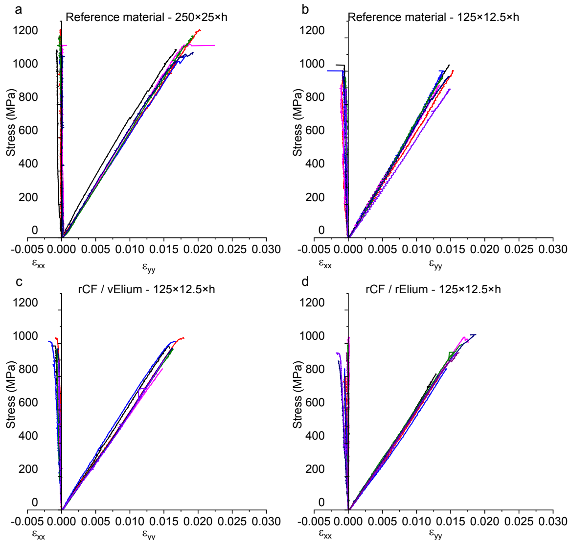
Figure 3-13: Uniaxial quasi-static tensile stress-strain curves of 0^\circ/90^\circ specimens of : (a) reference 250 \times 25 samples, (b) reference 125 \times 12.5 samples, (c) rCF/vElium and (d) rCF/rElium
