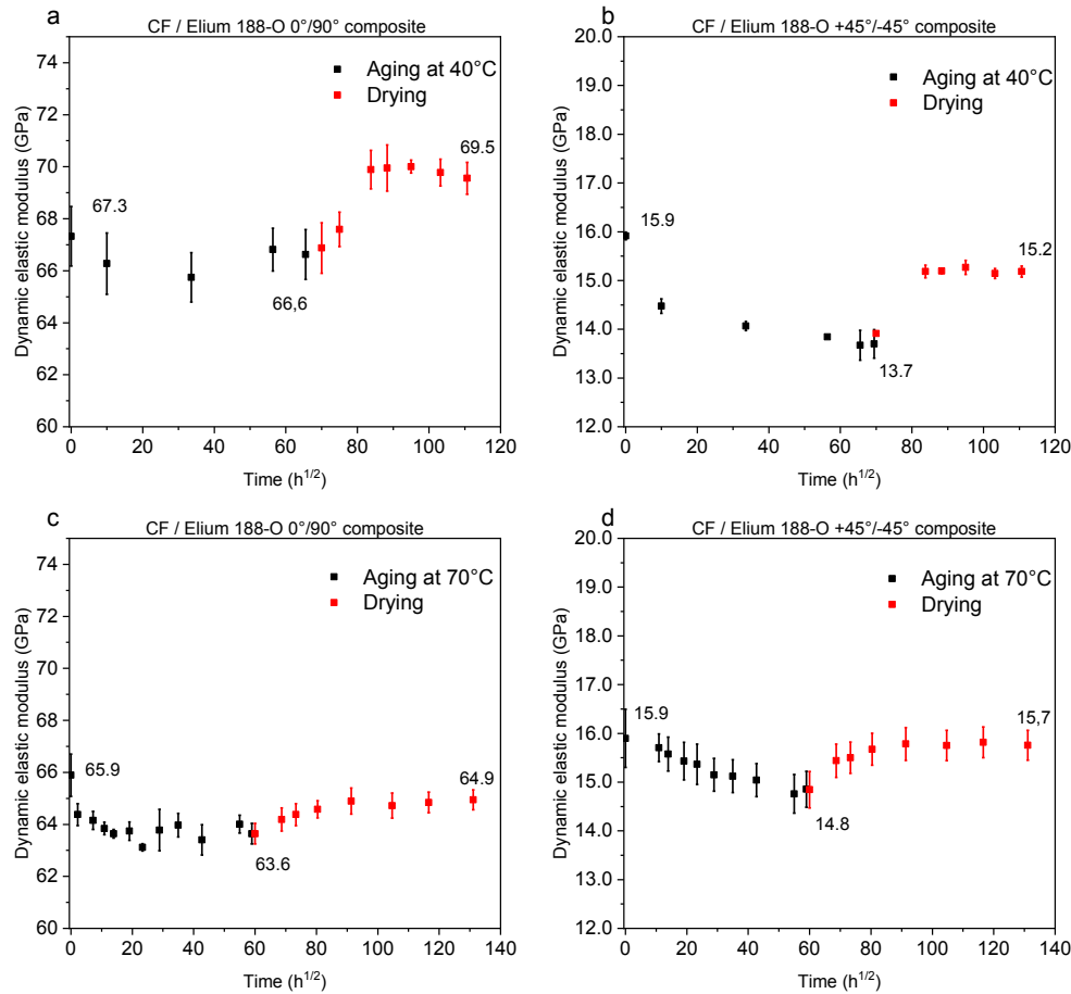
Figure 2-23: Modal analysis results represented by dynamic elastic modulus performed on [0/90]_4 and [+45/-45]_4 samples at reference (unaged), aged at 40 °C (a, b) and 70 °C (c, d) and dried after aging
