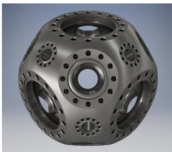
Figure 2.5: Main chamber.
