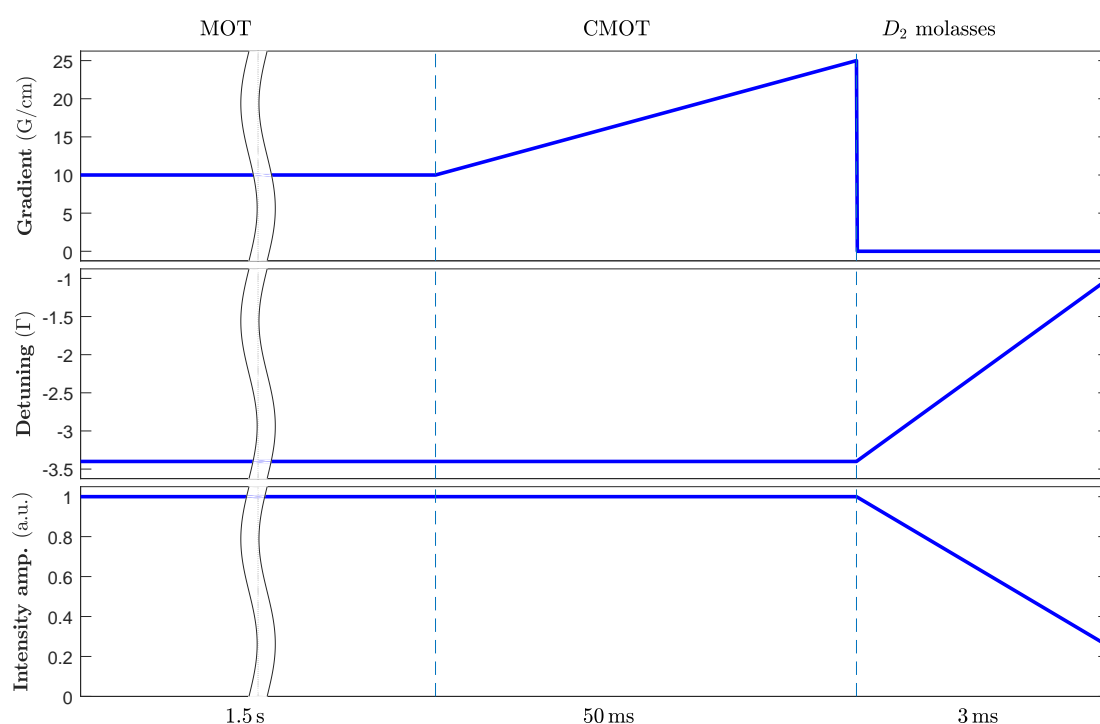
Figure 3.5: The sequence of MOT loading, CMOT and D_2 molasses.
