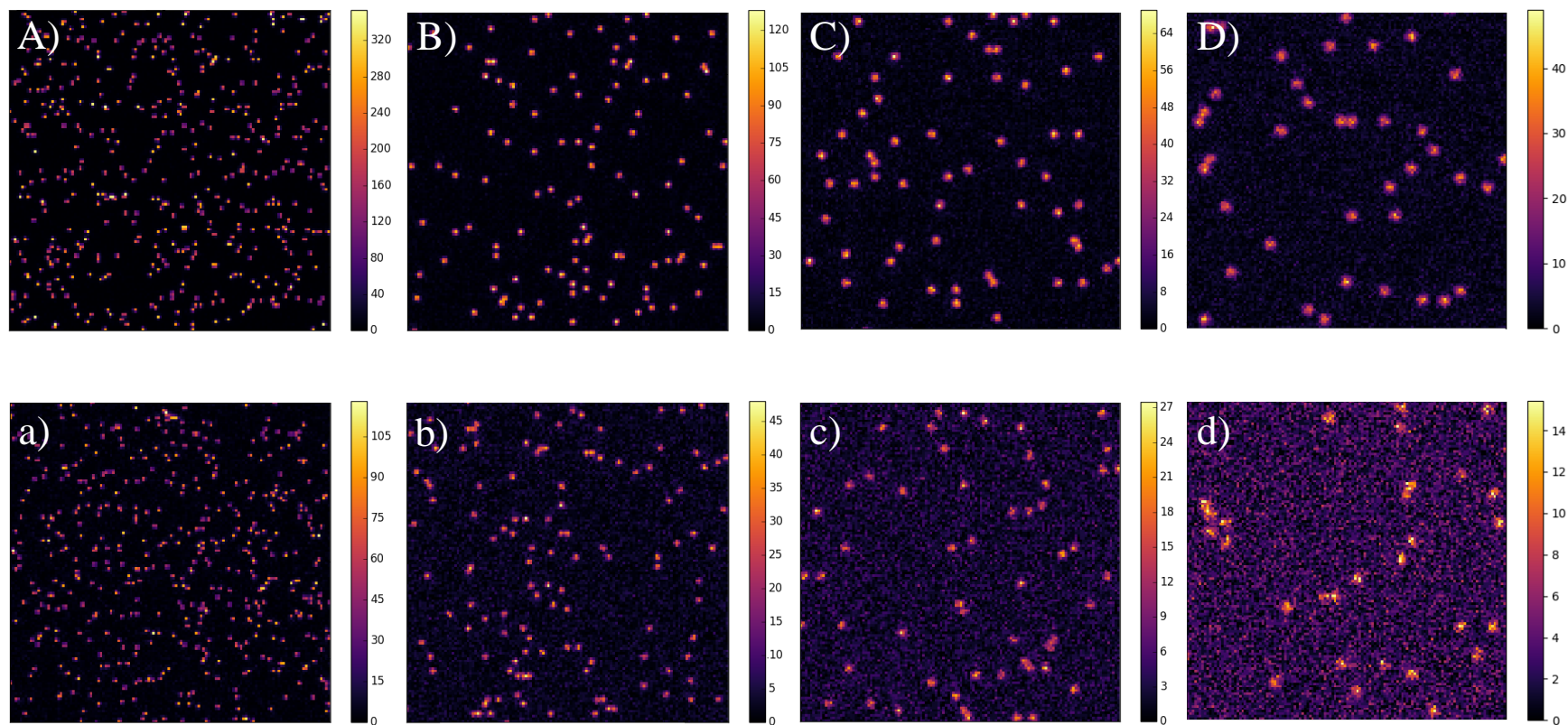
Figure 6.5: Simulated images for different magnifications and number of photons collected per atom. The whole camera chip is composed of 1700 \times 1700 pixels. A)-D): for 500 photons collected per atom, with a magnification of M = 20 (A), M = 40 (B), M = 60 (C) and M = 80 (D). a)-d): The same magnification values but for only 150 photons collected per atom. The noise level here is purely the statistical noise due to photon counts. Pictures taken from [135].
