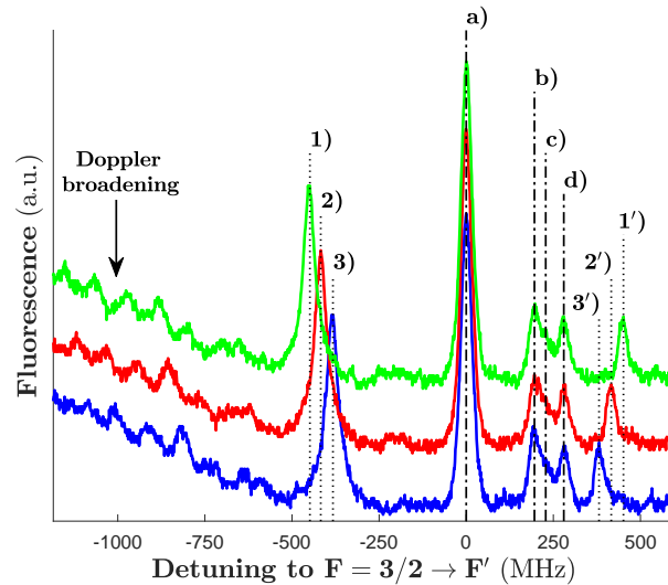
Figure 3.4: The Zeeman slower while functioning with current I = 16.7\text{ A} . The lines resulting from the perpendicular beam: a), b), c) and d). The angle between the perpendicular beam and the atomic jet gives the calibration ratio for detuning and speed v/\delta = 0.82\text{ (m/s)/MHz} . From the green line to the blue line, the exit velocity of the atomic jet decreased by 55 m/s.
