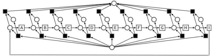
Figure 5.6: Round-robin.
