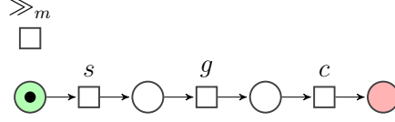
Figure 4.6: The net ((N_\sigma)^{\gg_m}) Used to Produce the Words \sigma^{\gg_m} for a Log Trace \sigma = \langle s, g, c \rangle .
