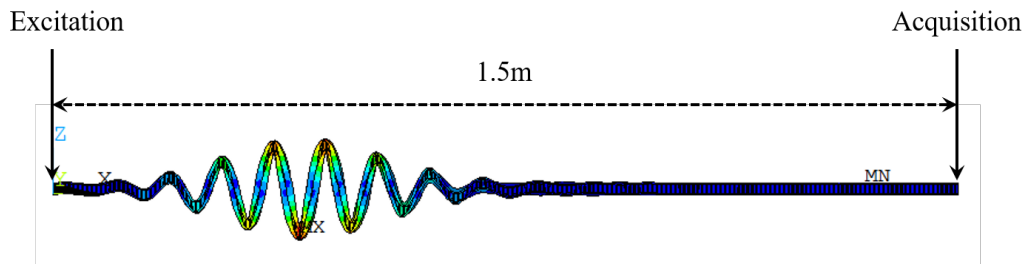
Figure 2.6: Illustration of the beam for the measurement of group velocity in direction x . The length is L=1.5\text{m} . Excitation signal is a pulse of frequency 4000\text{ Hz}
