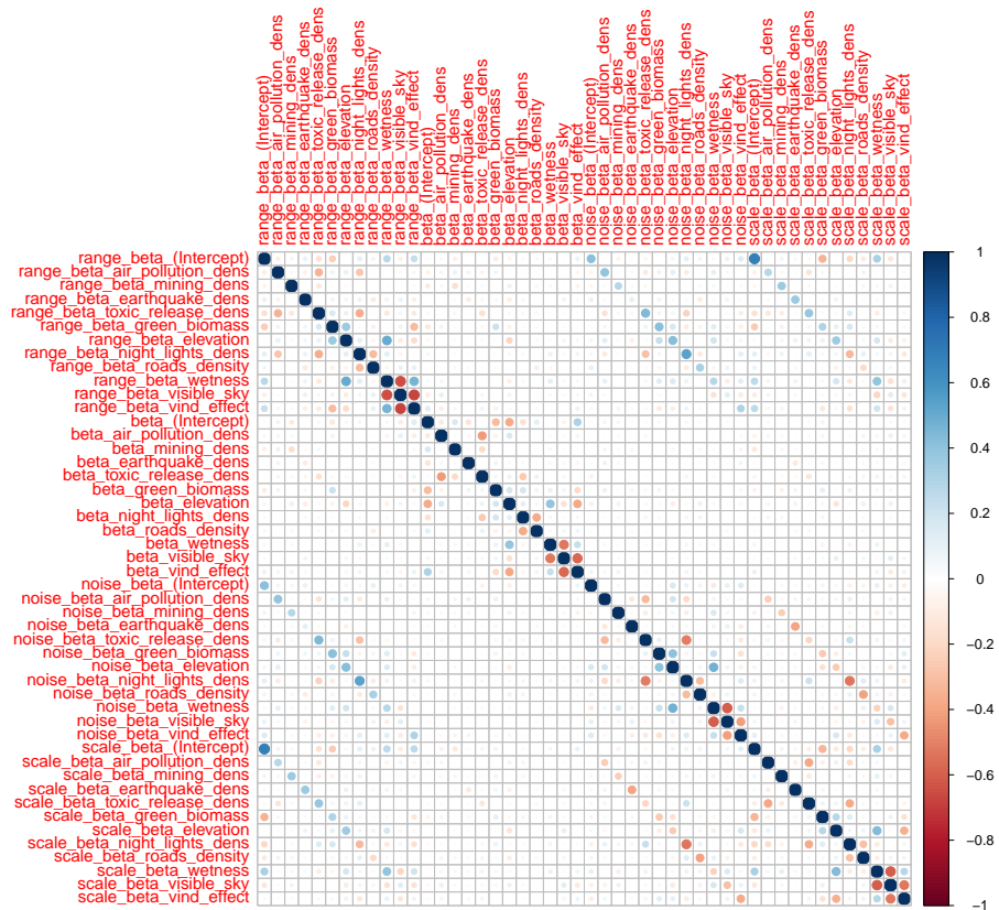
Figure 4.12: Correlation plot of the high level parameters for the lead data set analysis
