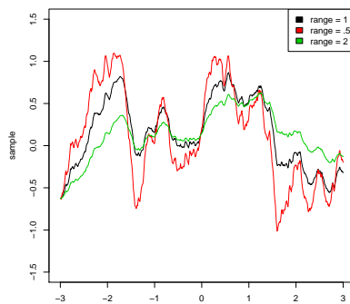
(d) Gaussian Process samples with varying range
