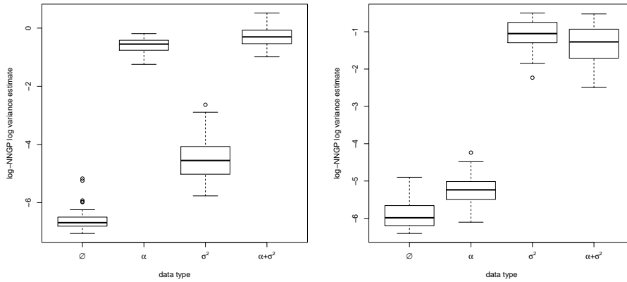
(a) Estimates of the log variance for w_\alpha (b) Estimates of the log variance for w_\sigma
