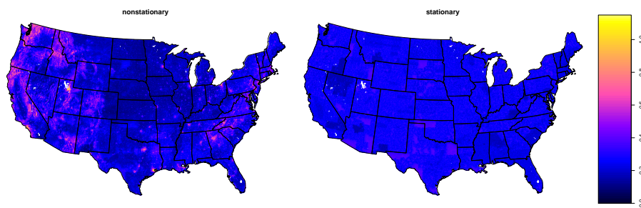
Figure 4.7: Predicted latent standard deviation of the lead concentration
