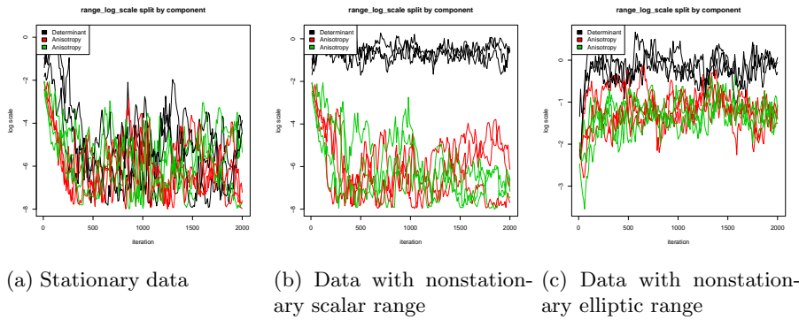
Figure 4.3: Log-scale analysis of the matrix log-NNGP prior of the range parameter
