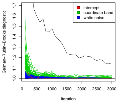
(c) \hat{R} of our implementation
