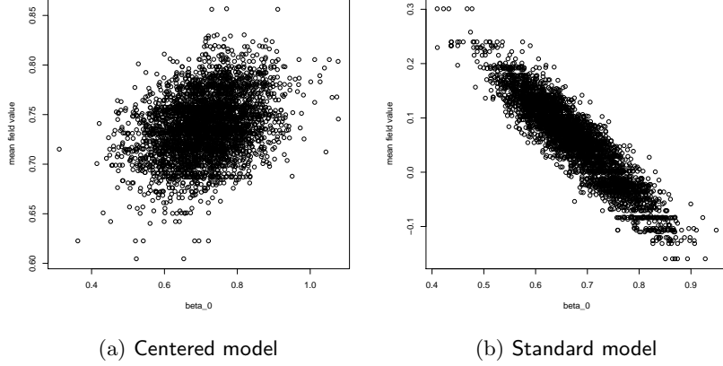
Figure 3.2: When plotting \frac{1}{n}\Sigma w(\mathcal{S}) against \beta_0 , the standard model exhibits a ridge-shaped point cloud
