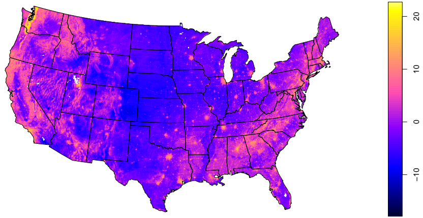
Figure 4.5: Visualization of the spatial incoherence of the lead measurements
