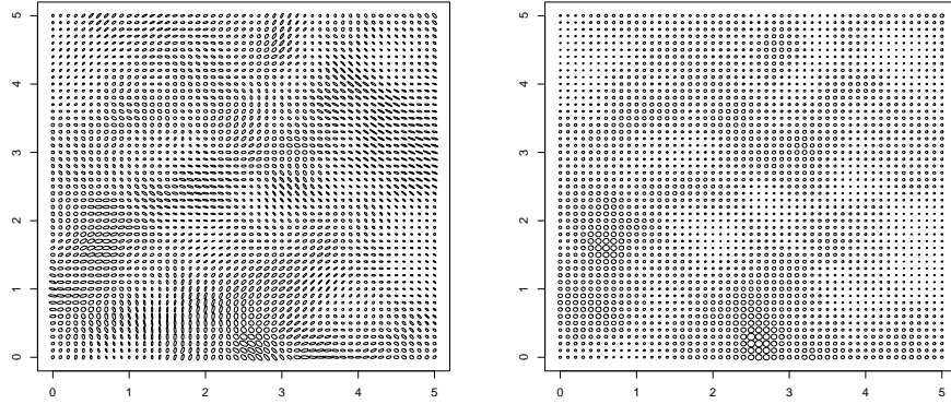
(a) Ellipses obtained with matrix log-NGGP (b) Circles obtained with scalar log-NGGP
