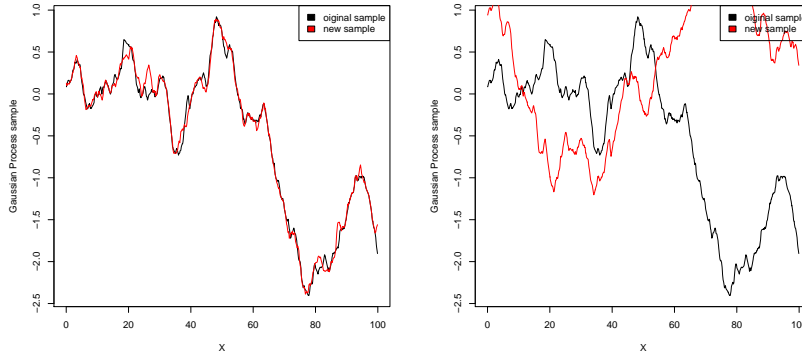
(a) Changing the 900 last coeff. of w^* (b) Changing the 100 first coeff. of w^*
