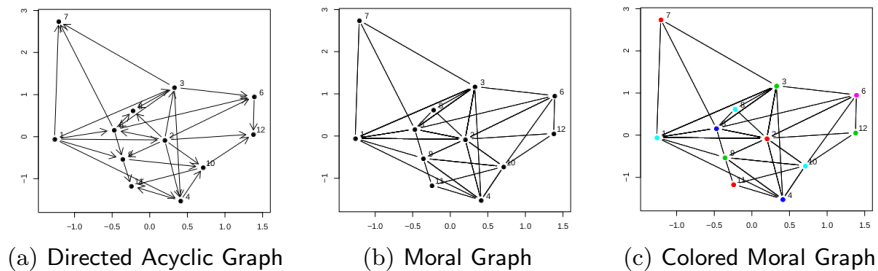
Figure 3.3: Moralization and coloring of a DAG
