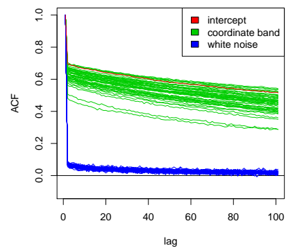
(f) Autocorrelations with spNNGP
