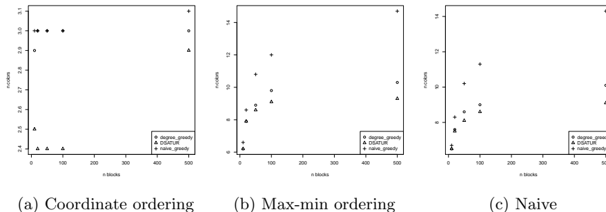
Figure 3.8: Number of colors following the number of blocks, for spatial domain dimension d = 2 and number of parents m = 5 .
