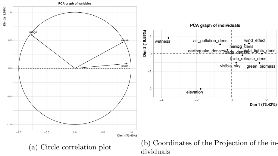
Figure 4.11: PCA of (\beta_\alpha | \beta_{\sigma^2} | \beta_{\tau^2})
