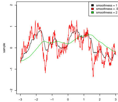
(b) Gaussian Process samples with varying smoothness
