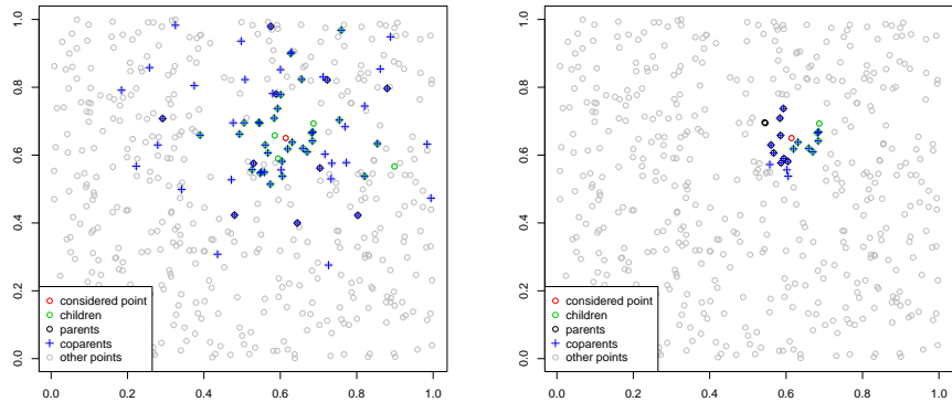
(a) Max-min ordering (the considered point is the 30 th of 500)
