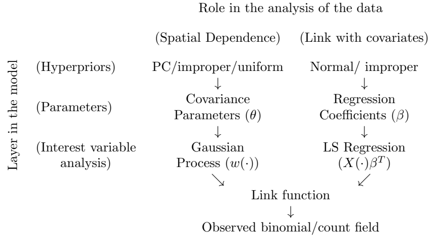
Figure 1.2: Schema of a hierarchical generalized space-time GP model
