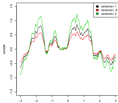
(f) Gaussian Process samples with varying marginal variance
