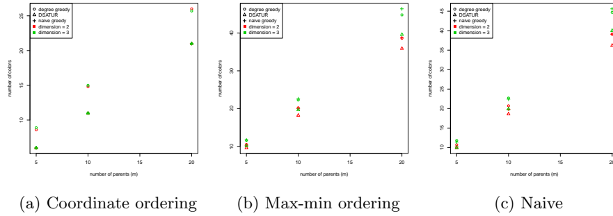
Figure 3.6: Impact of the spatial domain dimension and the coloring algorithm on the mean number of colors, for graphs of size n = 2000 .
