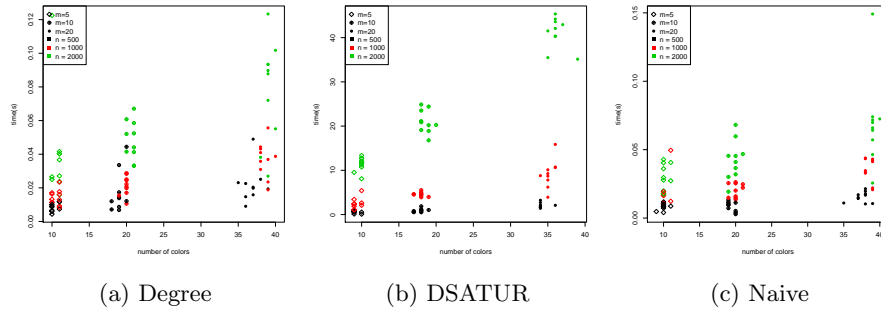
Figure 3.7: Repartition of the number of colors and running time with random ordering and d=2 .
