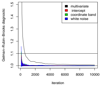
(a) \hat{R} with response spNNGP
