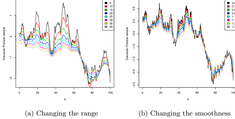
Figure 2.2: Effect of a change of covariance parameters on a Matérn latent field with fixed ancillary augmentation
