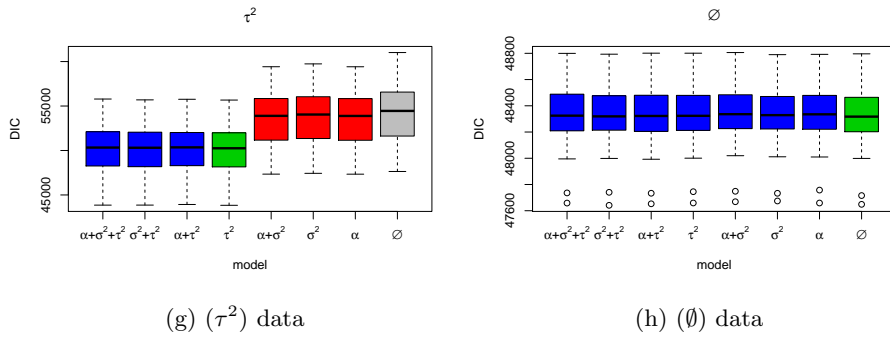
Figure 4.8: DIC of the models following the data Legend: “right model” ■; “wrong model” ■; “over-modeling” ■; “under-modeling” ■
