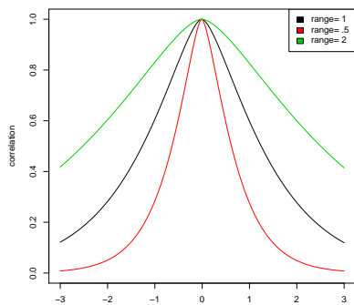
(c) Matérn covariance functions with varying range
