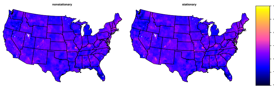
Figure 4.6: Predicted latent mean of the lead concentration
