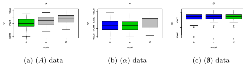
Figure 4.9: DIC of the models following the data, in the anisotropy model Legend: “right model” ■; “over-modeling” ■; “under-modeling” ■
