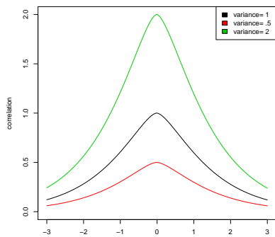
(e) Matérn covariance functions with varying marginal variance
