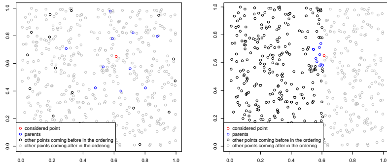
(a) Parents of a point with max-min ordering (30 th of 500) (b) Parents of a point with coordinate ordering
