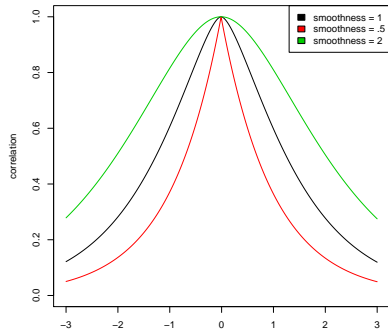
(a) Matérn covariance functions with varying smoothness
