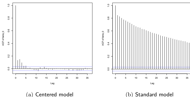
Figure 3.1: The ACF of \beta_0 drops much faster in the centered model than in the standard model
