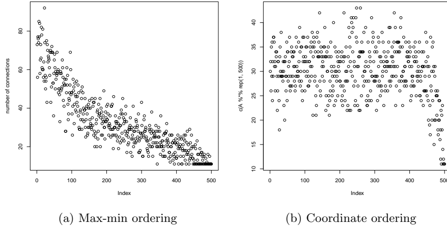
Figure 3.5: Number of connections of a point given its place in the ordering (same graphs as in figure 3.4)
