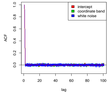
(b) Autocorrelations with response spNNGP
