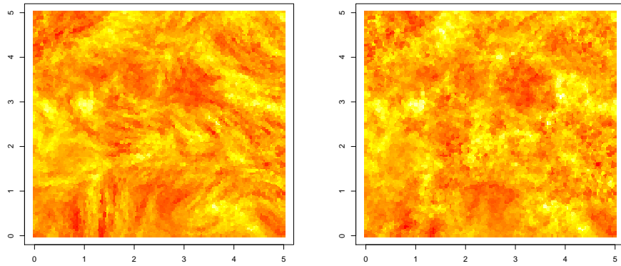
(c) NNGP samples corresponding to the ellipses (d) NNGP samples corresponding to the circles
