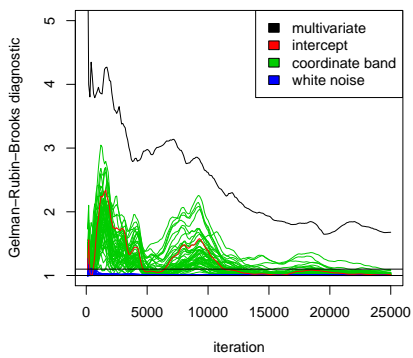
(e) \hat{R} with spNNGP
