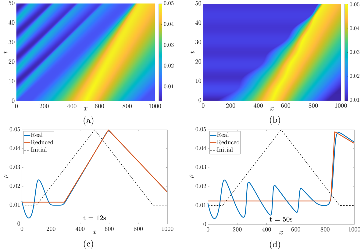
Figure 3.5: Comparison of real and reduced solutions to the LWR equation (3.29) with \phi_{in}(t) = 0.2 + 0.15 \sin(t/2) vehicles per second. (a): Evolution of real density \rho(t, x) . (b): Evolution of approximated density \hat{\rho}(t, x) . (c): Comparison of densities at t = 12 s. Real density \rho(t, x) is shown with blue line, approximated density \hat{\rho}(t, x) with red line and initial density \rho_0(x) with black dashed line. (d): Comparison of densities at t = 50 s.
