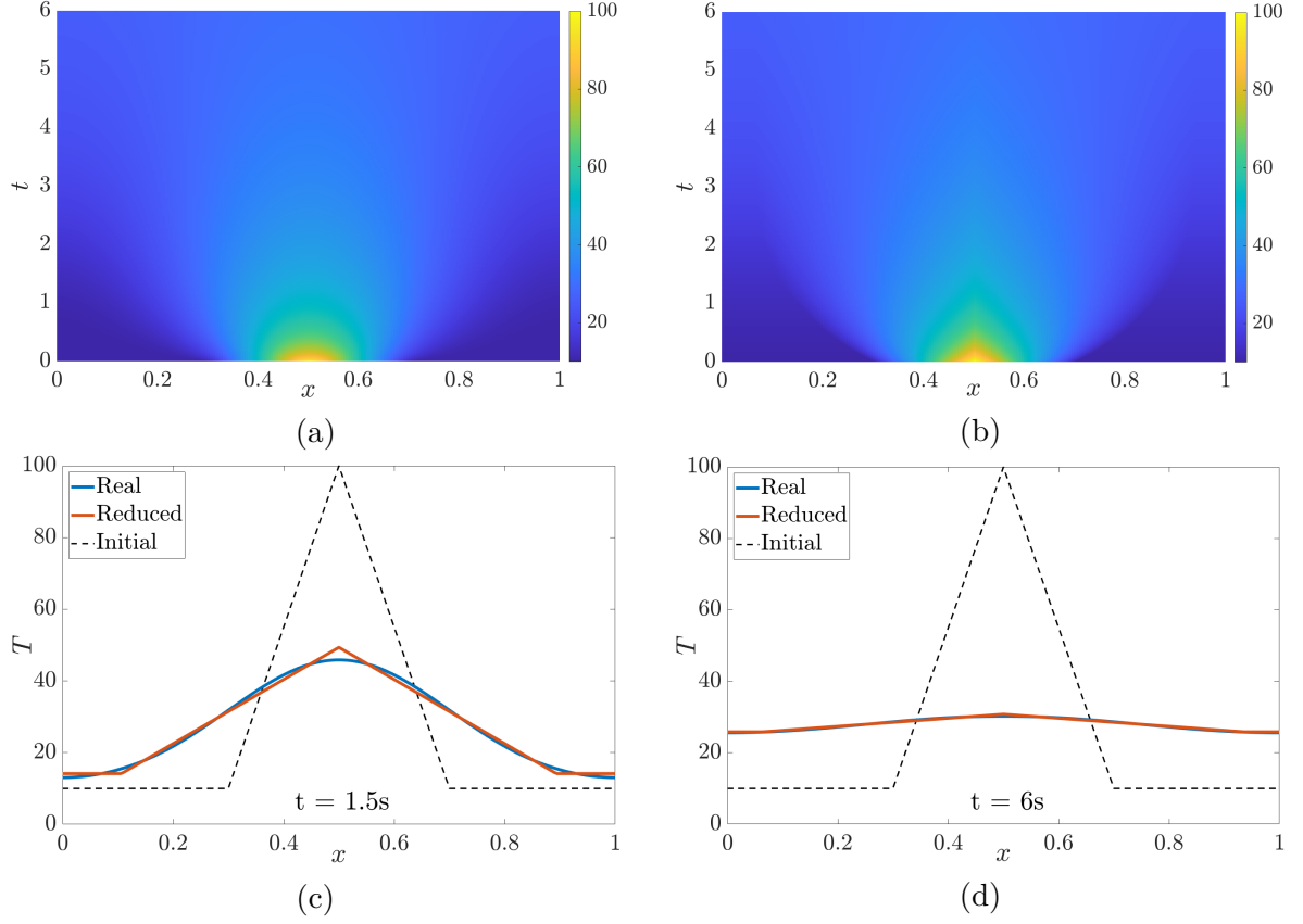
Figure 3.3: Comparison of real and reduced solutions to the heat equation (3.34) for the temperature of a copper rod in Celsius assuming the system is closed: \phi_{in} = \phi_{out} = 0 K·m/s. (a): Evolution of real temperature \rho(t, x) . (b): Evolution of approximated temperature \hat{\rho}(t, x) . (c): Comparison of temperatures at t = 1.5 s. Real temperature \rho(t, x) is shown with blue line, approximated temperature \hat{\rho}(t, x) with red line and initial temperature \rho_0(x) with black dashed line. (d): Comparison of temperature at t = 6 s.
