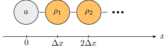
Figure 4.6: Boundary of the system (4.48) with Dirichlet boundary condition (4.49), represented by a ghost cell \rho_0 = a .
