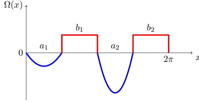
Figure 6.7: Intervals of loads and generators with generators designed according to the Proposition 6.2 with Remark 6.1. \Omega(x) on intervals b_j is an average of the neighbouring loads.
