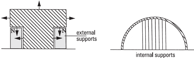
Fig. 2.15. The examples of internal or external support [107].
