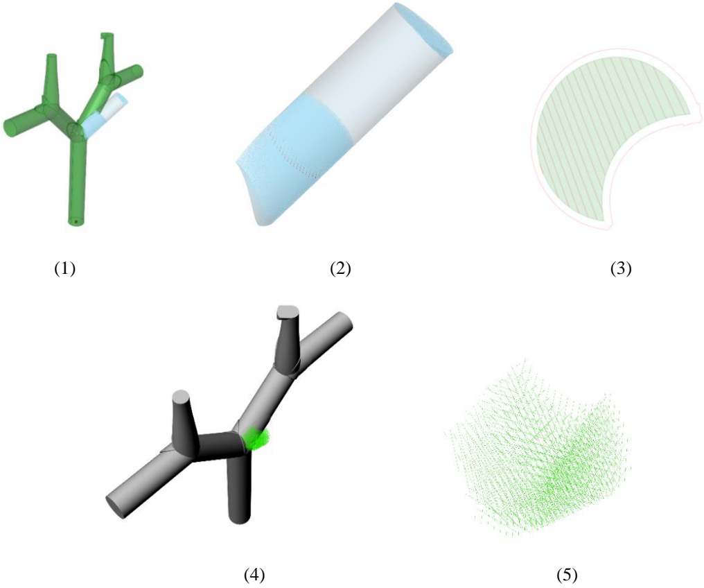
Fig. 3.37. (1). The fist subparts with the path; (2), (3). One layer is selected to show the details of toolpath; (4), (5). Several layers of the first subpart.
