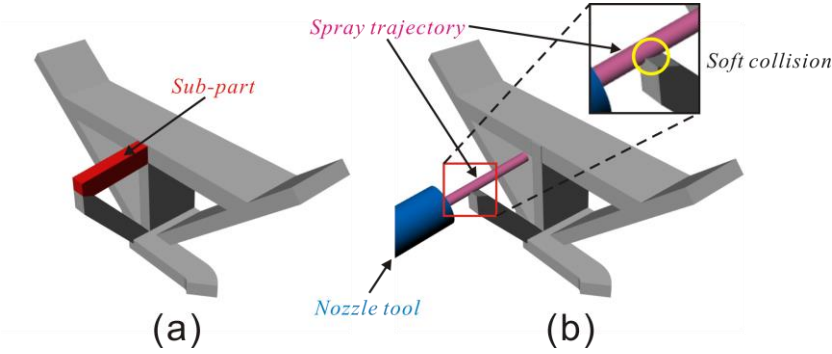
Fig. 4.28. The soft collision in case 3.
