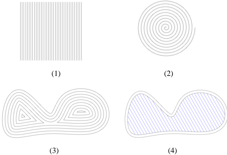
Fig. 2.19. Some typical toolpaths: (1) the rastering; (2) the spiral; (3) the offset; (4) the combination of more than one types.
