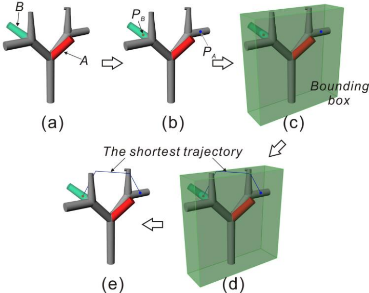
Fig. 3.23. The bounding box of initial volume with existing subparts: (a). Subpart A has been manufactured; (b). PA and PB are tip points of tool; (c). The bounding box envelop subpart A and existing initial volume; (d), (e). The tool move from PA to PB on the surface of bounding box and trajectory is a line when the box is unfolded to plane.
