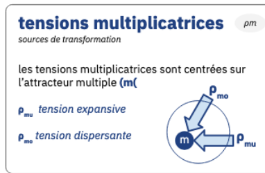
C43 – [\rho_m] – tensions multiplicatrices
