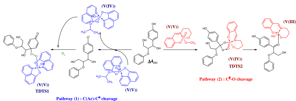
Figure IA. 10: Two examples of interactions between the substrate \underline{A4}_{HH} and a V-catalyst [90]
