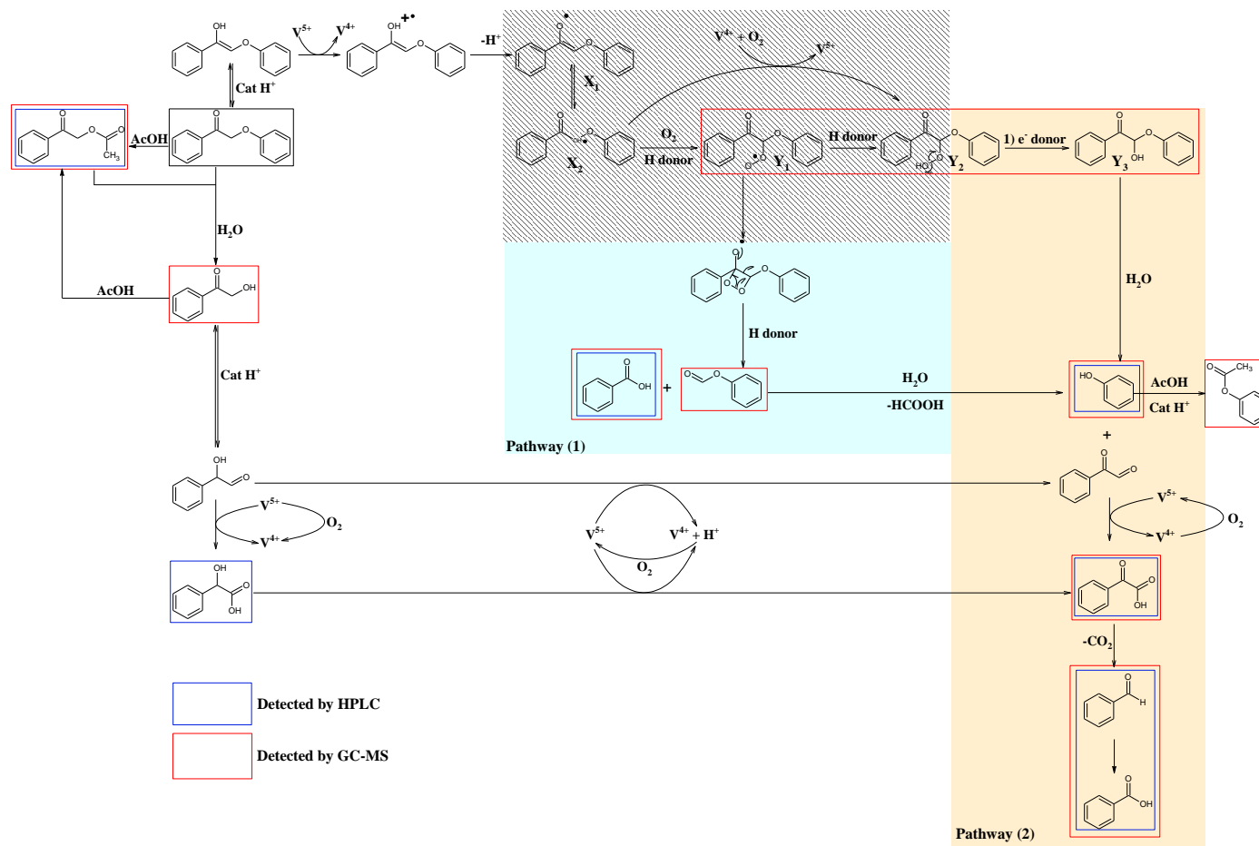
Figure II. 18: Mechanism proposal for the V3-HT catalyzed aerobic cleavage of K1_{HH}
