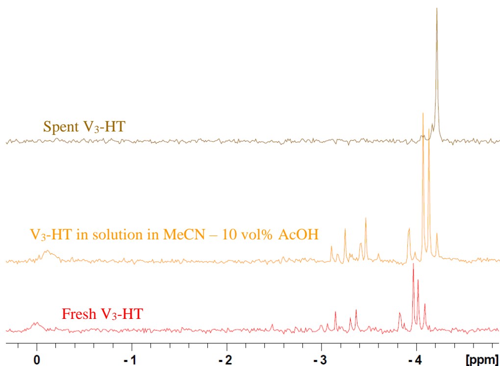
Figure II. 19: 31 P NMR spectra of the fresh and spent V 3 -HT catalysts (catalyst 30 mg in D 2 O-H 2 O 50:50 500 μL + dioxane 7.5 μL)
