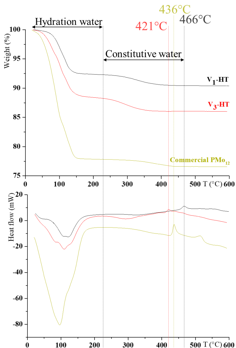
Figure II. 11: TGA-DSC profiles of \text{V}_x\text{-HT} (vs commercial \text{PMo}_{12} )
