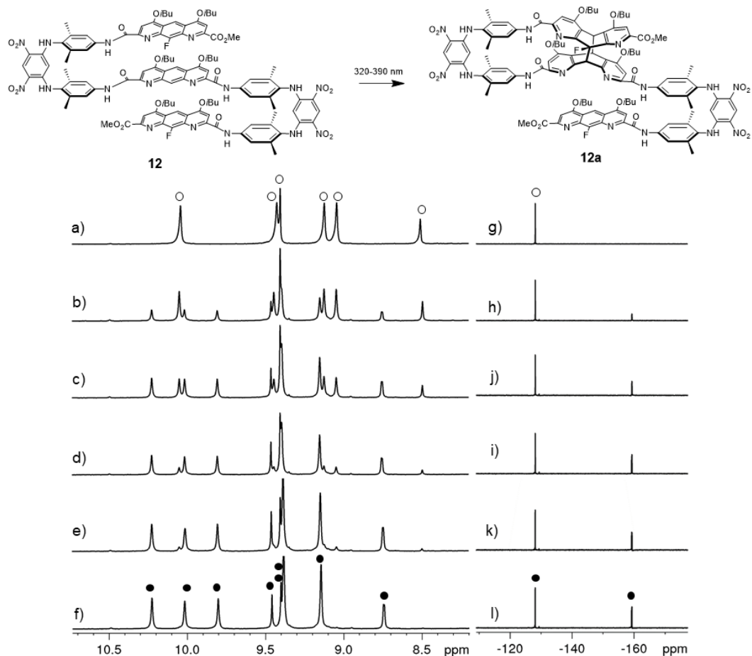
Figure 25. Schematic representation of photoirradiation (320 nm – 390 nm) induced adduct formation between two diazaanthracene (A F and A H ) units in 12 to 12a . Part of the 400 MHz 1 H NMR spectra of 12 at 298 K (1 mM in CDCl 3 ) under photoirradiation after (a) 0 min; (b) 15 min.; (c) 30 min; (d) 45 min; (e) 60 min; and (f) 75 min. The corresponding 376 MHz 19 F NMR spectra are given in (g) to (l), respectively. The signals correspond to the starting oligomer 12 are shown in empty cycles and for photoproduct, 12a , in black cycles.
