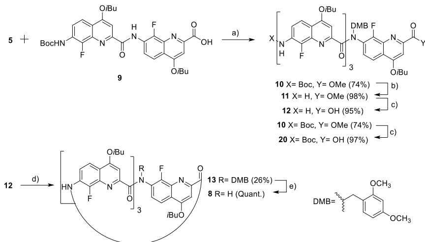
Scheme 3. Synthesis of Q^F tetramer 13 : a) i) 1-chloro-N,N,2-trimethyl-1-propenylamine, \text{CHCl}_3 , room temperature, 3 h; ii) DIEA, \text{CHCl}_3 , room temperature, 12 h; b) HCl 4N in dioxane, room temperature, 4 h. c) LiOH, THF, \text{H}_2\text{O} , room temperature, 4 h; d) triphenylphosphine, trichloroacetonitrile, DIPEA, \text{CHCl}_3 , room temperature, 48 h; e) trifluoroacetic acid, \text{CHCl}_3 , 60^\circ\text{C} , 2 h.
