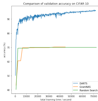
Figure 5.21 Comparison of GramNAS to DARTS and random search on CIFAR10. We see that the performance of random search and GramNAS are inferior to that of DARTS, at least before 70000 seconds. There is no significant difference between GramNAS and random search.
