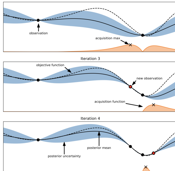
Figure 2.3 Bayesian optimization on real-valued functions. Figure from (Hutter et al., 2018).
