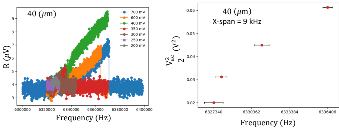
FIGURE 6.20: (left)Response of 41 μm string (right) Jump frequency against the square of the driving voltage
