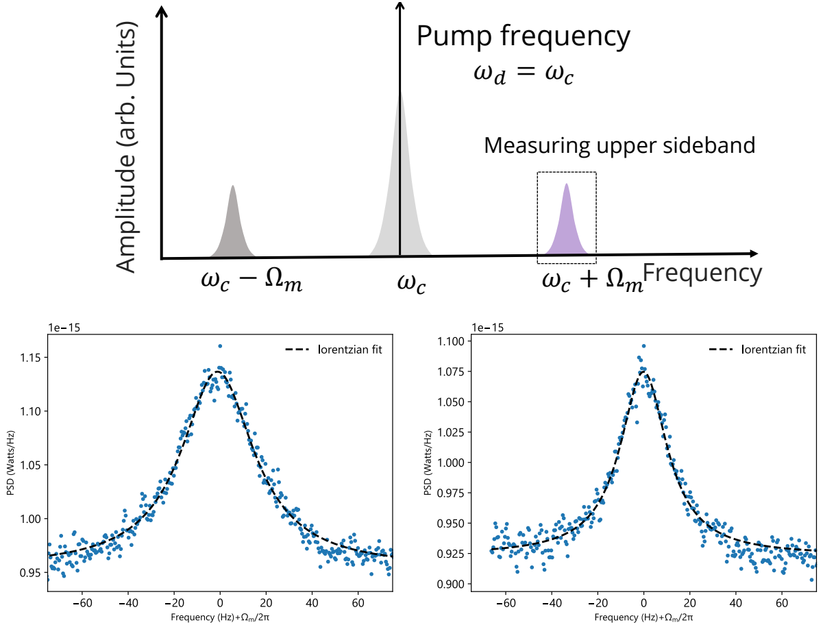
FIGURE 5.4: (upper) Sidebands generated at \omega_c \pm \Omega_m while pumping the MWC at \omega_c (bottom left) Mechanical sideband at \omega_c + \Omega_m at 500 mK (bottom right) Mechanical sideband at \omega_c + \Omega_m at 245 mK
