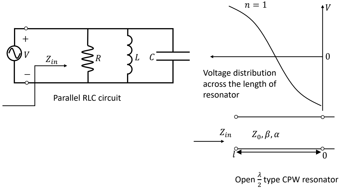
FIGURE 3.14: Voltage distribution across the length of open \frac{\lambda}{2} resonator for the fundamental mode. Voltage is maximum at the two ends of resonator. Also the resonator can be modeled as parallel RLC circuit
