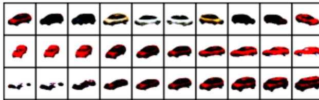
(b) CARS3D.
