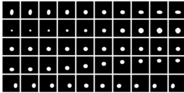
(a) DSPRITES.
