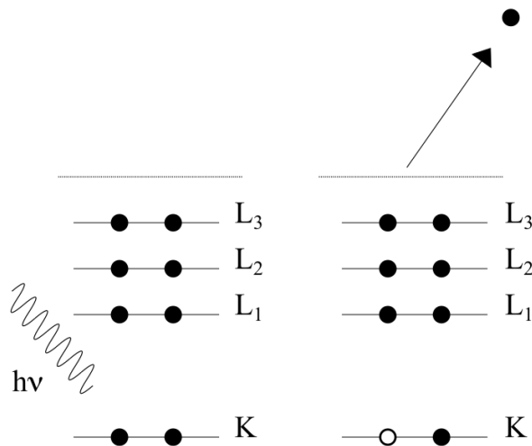
Figure 2.3 – Schematic representation of the photoemission process.
