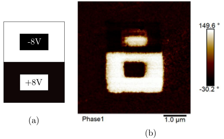
Figure 3.13 – PFM measurement performed on a 10 nm thick \text{BaTiO}_3/\text{Nb}:\text{SrTiO}_3 sample. (a) PFM written pattern and (b) PFM phase image in reading mode after writing the pattern pictured in (a).
