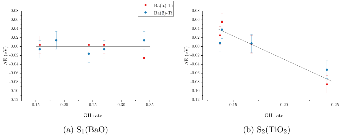
Figure 4.14 – Evolution of the shift Ba 4 d -Ti 3 p as a function of the hydroxyl concentration on the surface for (a) S_1(\text{BaO}) and (b) S_2(\text{TiO}_2) . The symbols are the same in both figures. The solid lines are only guides to the eye.
