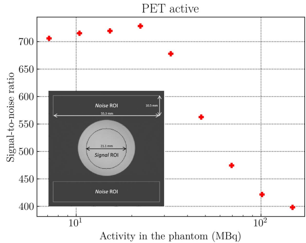
Fig. 13. SNR of spin echo images as a function of the activity in the phantom. SNR was defined complying to the ACR report, as shown on the screen capture on the left bottom corner of the graph.
