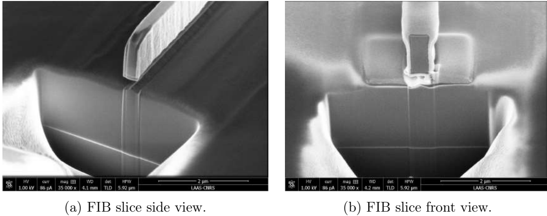
Figure 2.8: a. SEM image of a transistor fin FIB slice. It can be observed that the oxide underlying the fin has been completely etched. b. SEM image of a transistor fin FIB slice after the deposition of carbon and platinum layer for a better contrast.
