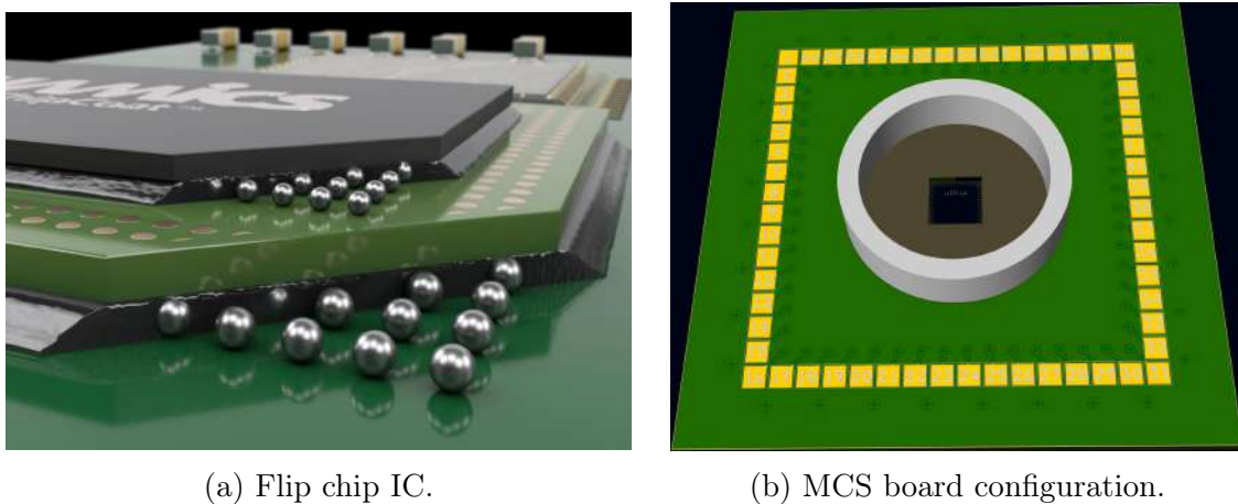
Figure 2.9: a. Examples of a flip chipped IC on a board with metallic bumps and underfill. Image taken from NAMICS website. b. CAD image of our PCB design compatible with standard available recording platforms.
