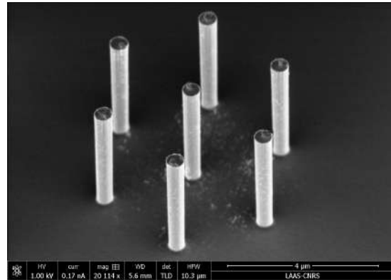
(c) Nanopillars.
