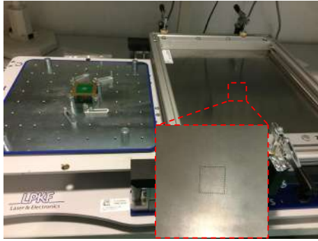
(a) Screen printing setup.
