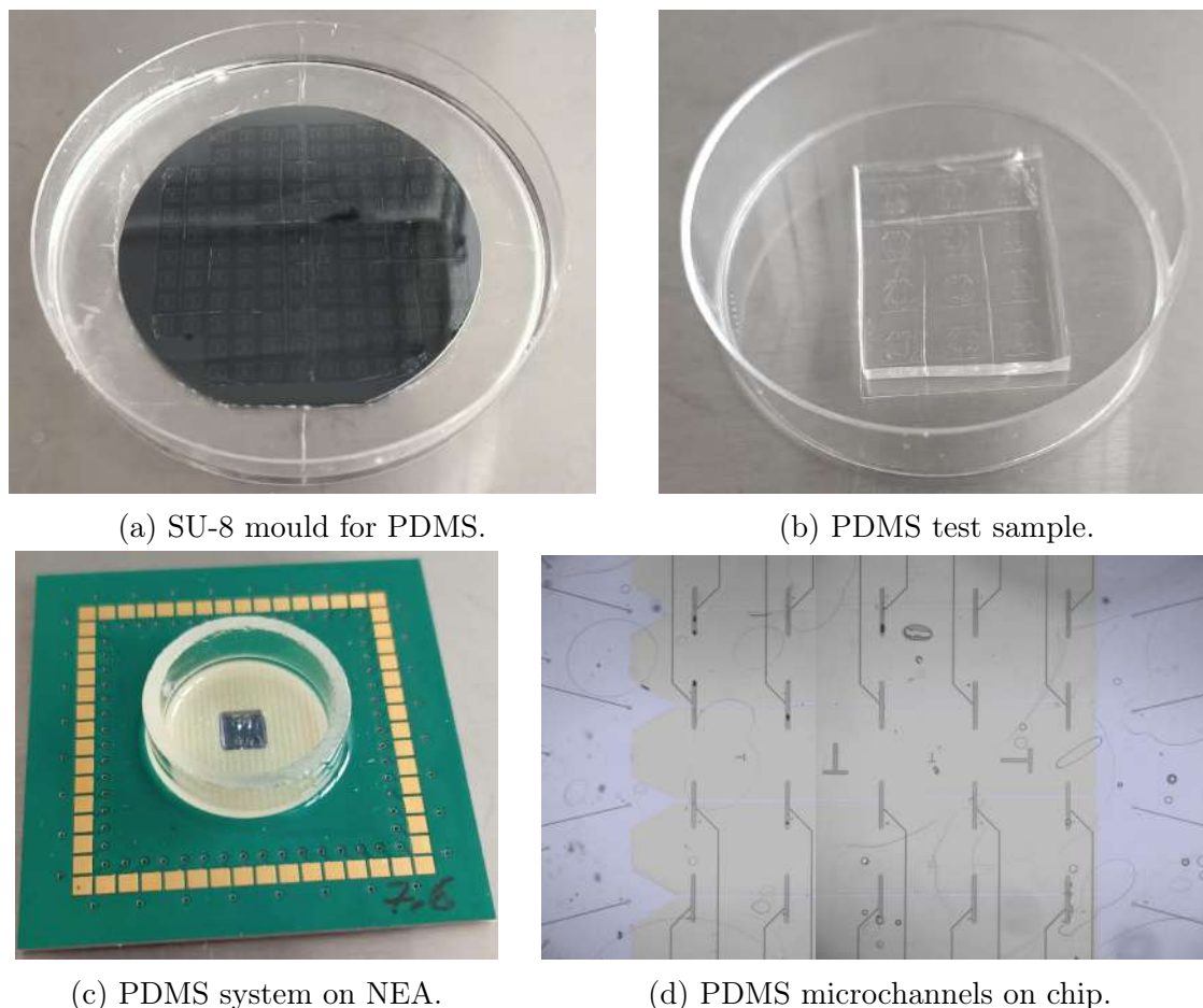
Figure 3.10: a. Photo of the SU-8 mould fabricated on a 4 inches wafer for PDMS microchannels. b. Photo of the test sample of the PDMS system bonded on glass coverslip. c. Photo of the complete NEA system with integrated PDMS microchannels system bonded on the chip. d. Colourized optical image by microscope of the PDMS microchannels aligned on NEA chip.
