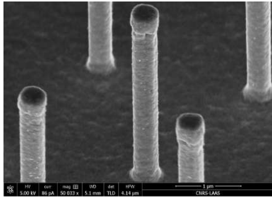
(b) PtSi nano pillars.
