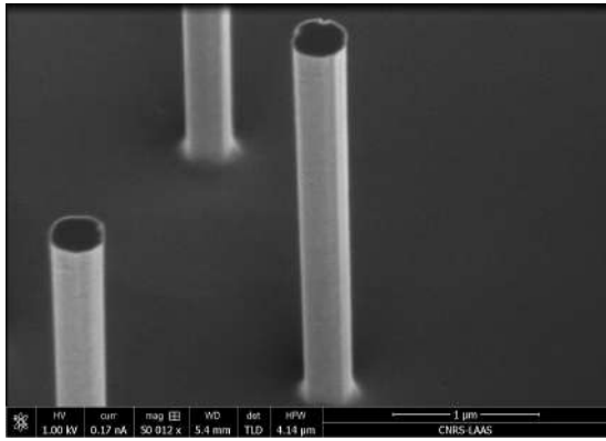
(a) Silicon nano pillars.
