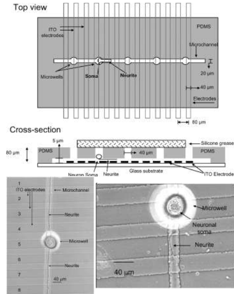
(b) Soma and neurites separation and recording.
