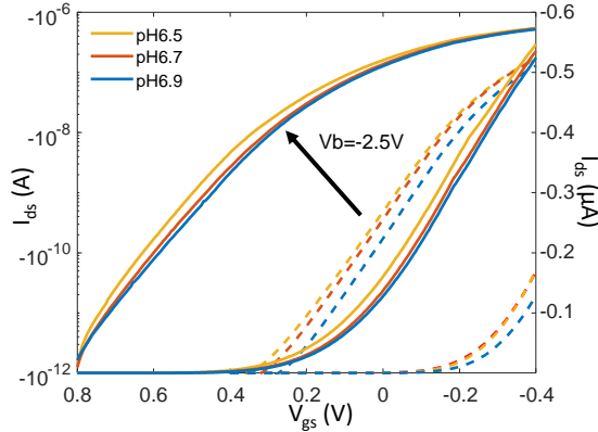
(a) ISFET characterization with ALD sensing layer and back-gate effect.
