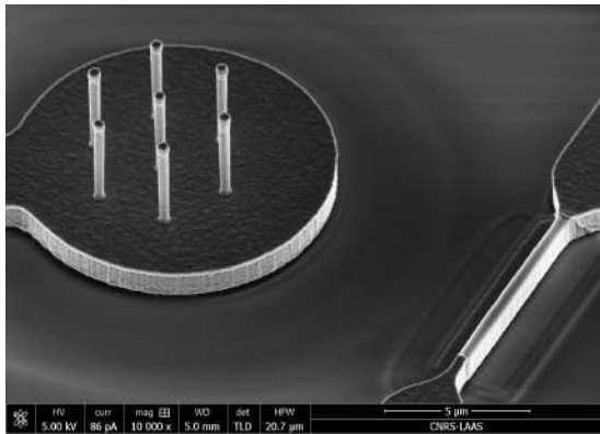
(a) Active and passive electrode.
