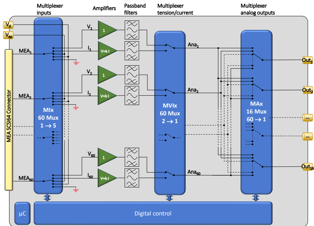
Figure 4.3: Schematic representation of the multiplexer PCB design. From left to right, the SCSI connection and two channels dedicated to electrical stimulation, the first multiplexer level (1 to 5 connections), the amplifiers and passband filter, the tension or current measurement switch and the final multiplexer level (60 to 1 connections).
