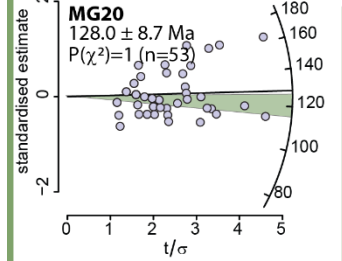
Figure 4.5 – Radial plots of single-grain AFT ages arranged according to the different sedimentary formations sampled for this study. Cretaceous samples from the Chubut Group clearly evidence a partial annealing of AFT data while Cenozoic samples show that no late heating affected those samples. Ages of deposition from Cuitiño et al., 2016, 2015b, 2015a; De Iuliis et al., 2008; Parras et al., 2012.
