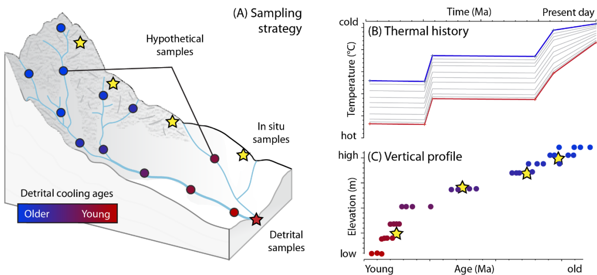
Figure 2.12 – Conceptual model to predict detrital distributions for thermochronological data (modified after Gallagher and Parra, 2020). (A) Comparison between typical in situ vertical profile, that may not cover the entire elevation range in catchment, and the modern detrital sample from the outlet for which a set of hypothetical dummy samples spanned over the total elevation range of the catchment. From a given specified thermal history (B) and the hypothetical samples, we can predict an age elevation profile (C) including kinetic parameters for FT (DPar). This allows to produce a set of AFT ages for the dummy samples at each elevation.
