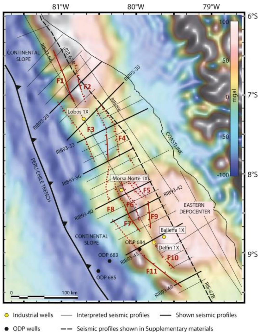
Fig. 2. Gravity map (Sandwell and Smith, 1997) from GeoMapApp (resolution: 1.75 \text{ km}^2 ) with the position of seismic lines interpreted in this study and wells used for chronology purposes (PARSEP, 2001). Faults are located after seismic interpretation.
