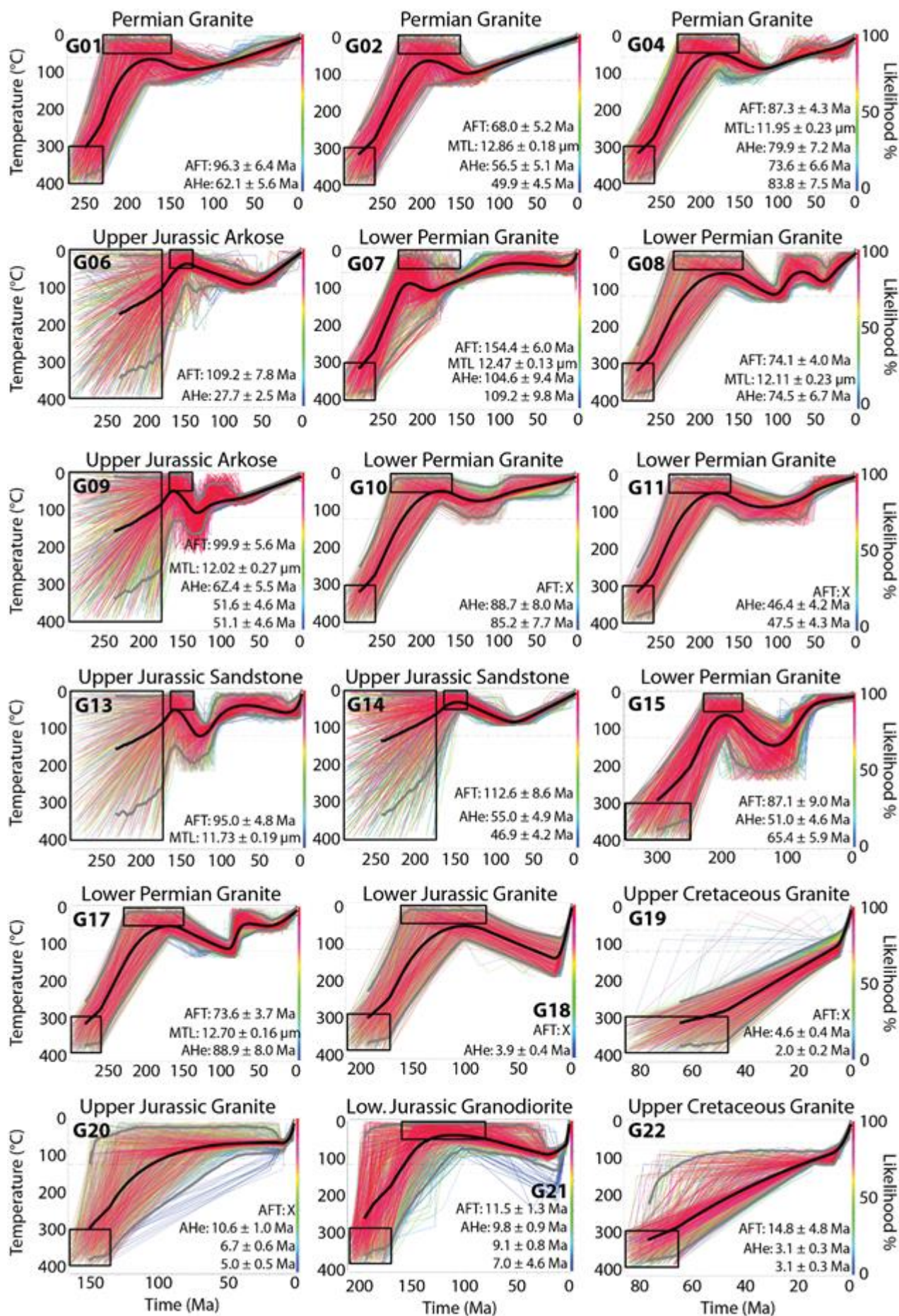
Figure 1a: Thermal history results from QTQt (samples G01 to G22).
