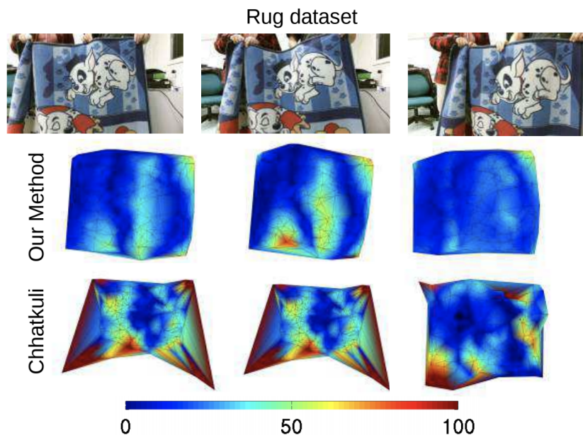
FIGURE 3.8: Example of estimates from Parashar et al. [112]. From top to bottom are: input images with deformable object wrapped over time, reconstruction error from [112] and reconstruction error from [32].
