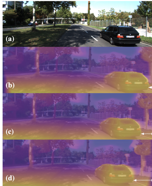
FIGURE 3.14: Poggi et al. qualitative evaluation. a) is the input image, b) and d) are respectively the left and right estimation while c) is the center (image-aligned) estimation.
