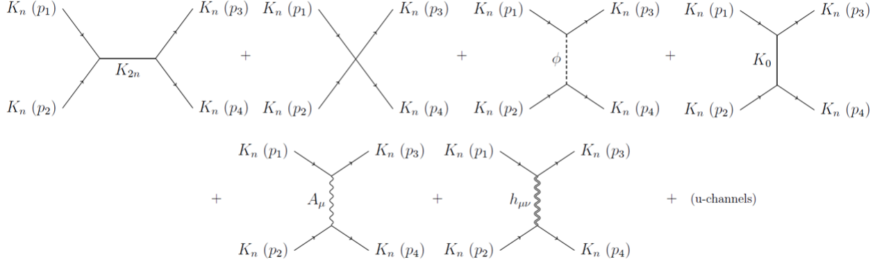
Figure 4.2 – Diagrams present in the \varphi_n \varphi_n scattering.
