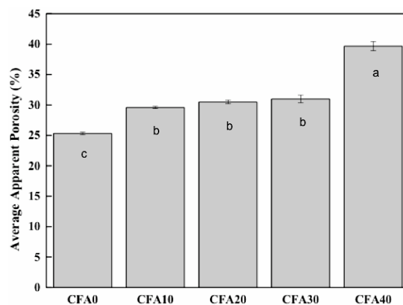
Figure 34 – Average apparent porosity percentage for the alumina-based tubular membrane incorporated with different CFA concentrations.
