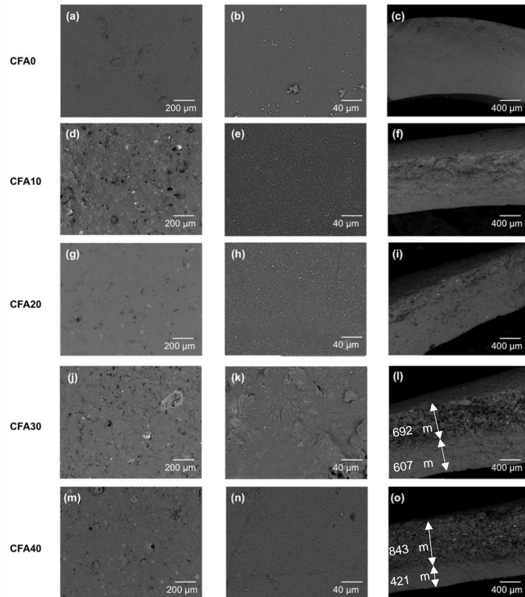
Figure 35 – SEM micrographs of alumina-based tubular membranes incorporated with different CFA concentrations: outer (a, d, g, j, m), inner (b, e, h, k, n) and cross-section (c, f, i, l, o).
