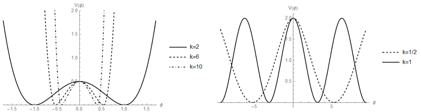
Figure V.1: Analytic extensions of the potential V(\phi) (V.18). The left panel displays the cases k = 2 , k = 6 and k = 10 , yielding a mexican hat-like profile; the right one, k = 1 and k = 1/2 , yielding a periodic profile.
