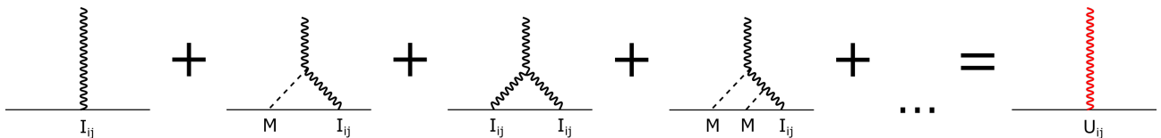
Figure III.3: Schematic dressing of the vertices of fig. III.2, for the quadrupolar moment. The ellipsis encompasses all higher non-linear interactions, building up to give the radiative moment U_{ij} .
