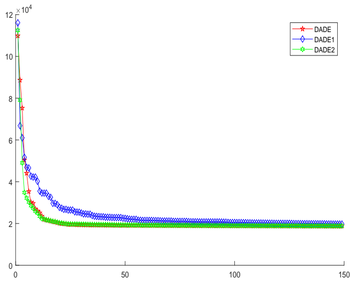
Figure 4.6: Convergence rate of DADE variants in function 14
