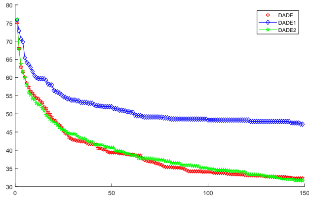
Figure 4.9: Convergence rate of DADE variants in function 21
