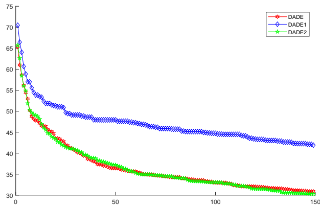
Figure 4.10: Convergence rate of DADE variants in function 22
