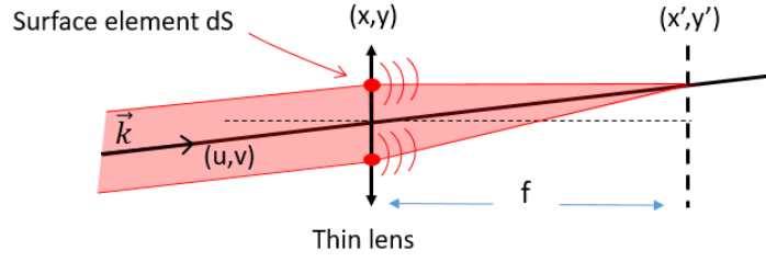
Figure B.3: Focusing of a plane wave into a point as explained in text. f is the focal length. \vec{k} wavevector at an angle u, v . dS = dxdy a surface element of a focusing lens
