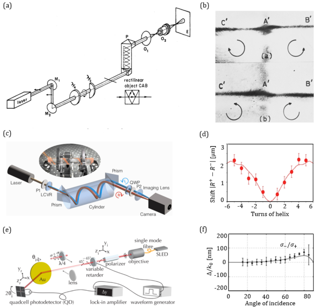
Figure 5.1: (a) Over-all experimental arrangement for measuring Imbert-Fedorov shift in circular polarization state. A laser beam, with horizontal linear polarization, traverses a quarter-wave plate and then a half-wave plate covering half of the beam; the resulting beam, which illuminates the rectilinear object CAB, is thus polarized circularly with opposite helicities on its two halves. This will produce the differential doubling effect we have alluded to. After illuminating the rectilinear object CAB, the beam enters either of our two multiplying prisms, and the image of CAB is finally observed. The high luminosity of the prism P allows this image to be projected on a screen. (b) Image of a rectilinear object displaying the transverse shift of a circularly polarized beam. The circular polarization states of the two halves of the beam are indicated. (See [20] for details). (c) Direct measurement of the spin-Hall of light in a glass cylinder in which the shift accumulates along a helical trajectory. (d) The relative shift between the two spin components versus the turns of the helix. (See [47] for details). (e) The optical set-up to measure the polarization-differential shift of a beam reflected off a thick gold film. (f) Measured polarization-differential shift between \sigma_-/\sigma_+ polarized light as function of the angle of incidence. (See [49] for details)
