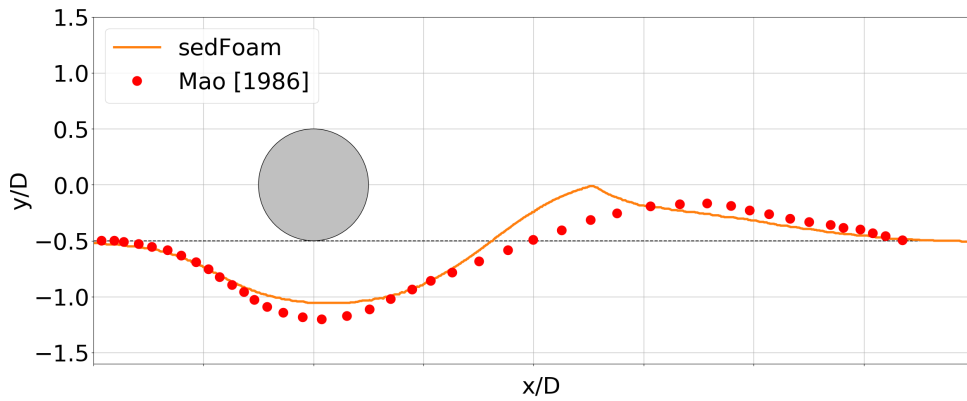
Fig. 2.2: Sediment bed profiles at 11s using a k - \epsilon turbulence model (Chauchat et al., 2017).
