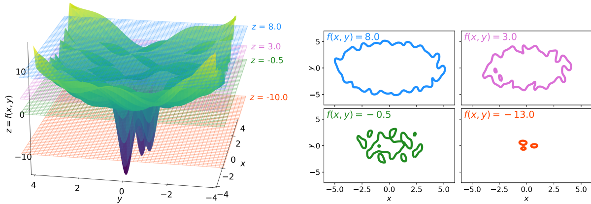
FIGURE 1.6: (Left) A generic “rough” landscape f(x, y) with several deep minima in dimension 2. (Right) Slices z = f(x, y) , shown as planes in the left picture. For z high enough (high energy, or high temperature by the microcanonical-canonical equivalence in the thermodynamic limit) the slices are well-defined by a single “pure state”. As the energy decreases the slices get disconnected, and for low enough energy they are concentrated around the location of the deep minima of f(x, y) . This low-dimensional view is merely an intuition and should not be considered as anything more.
