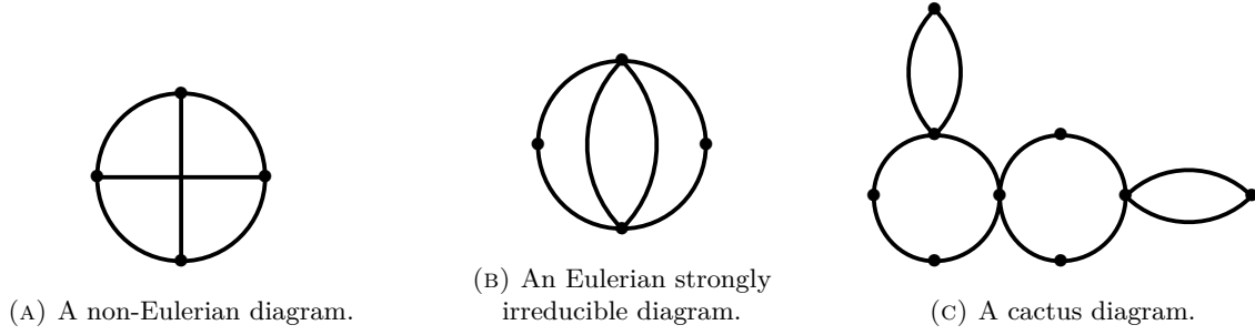
FIGURE 2.2: Cactus and non-cactus connected diagrams. Each vertex represents an index i over which we sum, and each edge is a factor J_{ij} . Each diagram carries a global factor n^{-1} .
