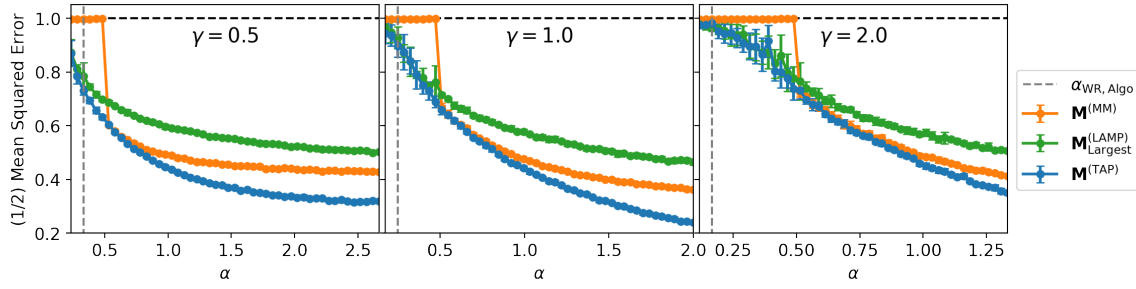
(A) Product of two real i.i.d. Gaussian sensing matrices with a size ratio \gamma \in \{0.5, 1.0, 2.0\} . The simulations were done using m = 10000 , and error bars are taken over 10 instances.
