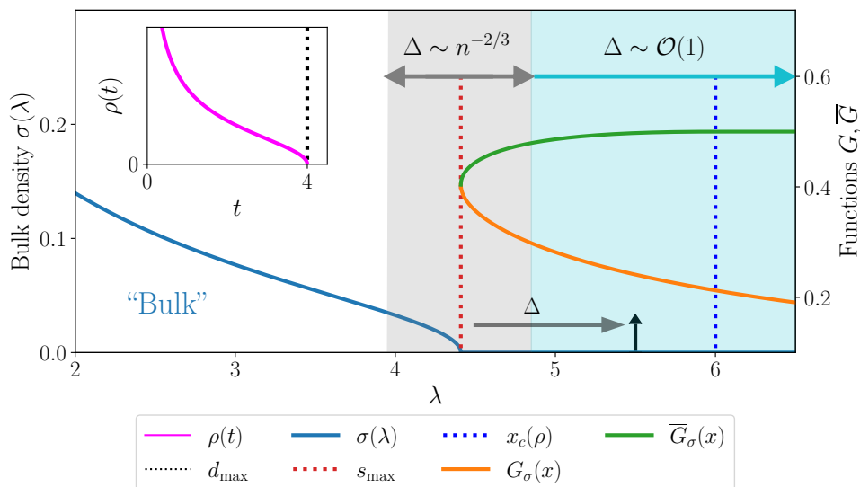
FIGURE 8.1: The bulk \sigma(\lambda) , and the functions G_\sigma, \bar{G}_\sigma for \alpha = 2 and \rho(t) the Marchenko-Pastur law with ratio 1. In the box, we plot \rho(t) and the right edge d_{\max} of its support. The black arrow is an outlier in the spectrum of \mathbf{H}_n , and \Delta is the gap between this outlier and the bulk \sigma(\lambda) . As we will see, the rate function of the large deviations of \lambda_{\max}(\mathbf{H}_n) is directly proportional to the area between G_\sigma and \bar{G}_\sigma .
