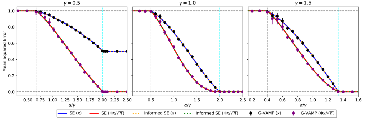
FIGURE 6.4: Mean squared error as a function of the measurement rate \alpha , for a sensing matrix \Phi = \mathbf{W}_1 \mathbf{W}_2 a product of two complex i.i.d. standard Gaussian matrices \mathbf{W}_1 \in \mathbb{C}^{m \times p} , \mathbf{W}_2 \in \mathbb{C}^{p \times n} with aspect ratios \gamma = p/n \in \{0.5, 1.0, 1.5\} . Red curves denote the recovery on \Phi \mathbf{X}^* / \sqrt{n} and blue curves on \mathbf{X}^* . Cyan dashed lines denote the full reconstruction threshold \alpha_{\text{FR,IT}} . The G-VAMP experiments were performed with n = 5000 , and the mean and std are taken over 5 instances.
