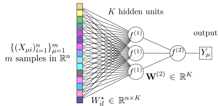
FIGURE 4.1: The committee machine is one of the simplest models of two-layers neural networks. Both activation functions f^{(1)}, f^{(2)} = \text{sign} and the second-layer weights \mathbf{W}^{(2)} are all fixed to 1. Here we represent a generic two-layers neural network with K = 3 .
