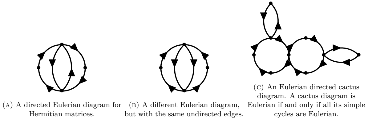
FIGURE A.2: Diagrams similar to the ones of Fig. 2.2, but for Hermitian matrices. Note that the diagrams of Fig. A.2a and Fig. A.2b are different because of the different directions of the edges, but that both are Eulerian.
