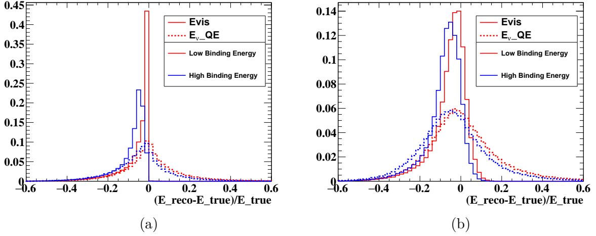
Figure 7.6: Comparison of reconstructed neutrino energy using E_{\text{vis}} (solid lines) and the CCQE formula using only muon kinematics (dashed lines). The different line colors indicate different values for the binding energy - 15 MeV, “low” (35 MeV, “high”) in red (blue). (a) Without detector smearing. (b) With SuperFGD smearing as described in Section 6.2.
