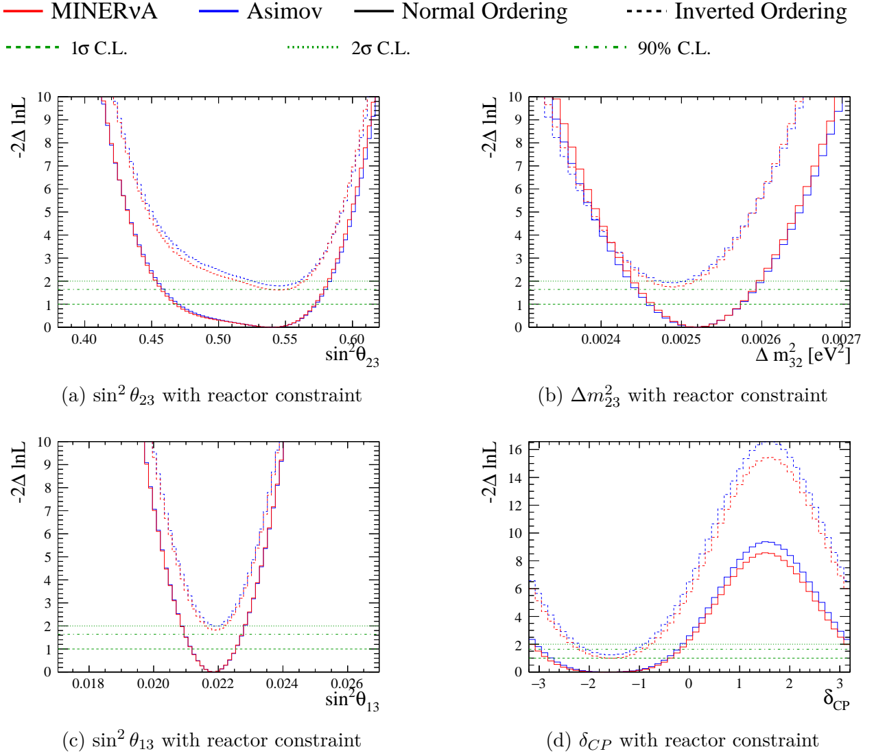
Figure 5.29: 1-D likelihood surfaces for all parameters, with the reactor constraint on \sin^2 \theta_{13} , assuming normal hierarchy for the MINERvA pion suppression tune simulated data set.
