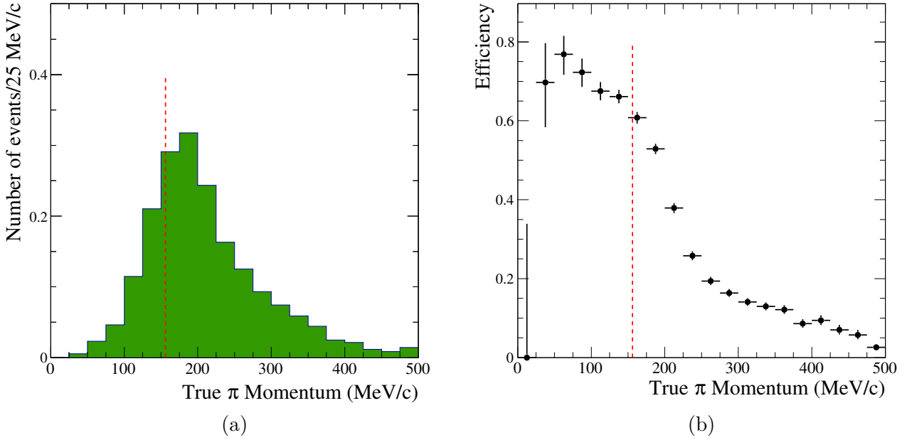
Figure 5.30: The true momentum distribution for selected simulated signal events in the 1Re1de sample with 1 electron-ring and 1 Michel electron at SK (a) and the selection efficiency for these events (b). The red dashed line indicates the Cherenkov threshold for charged pions.
