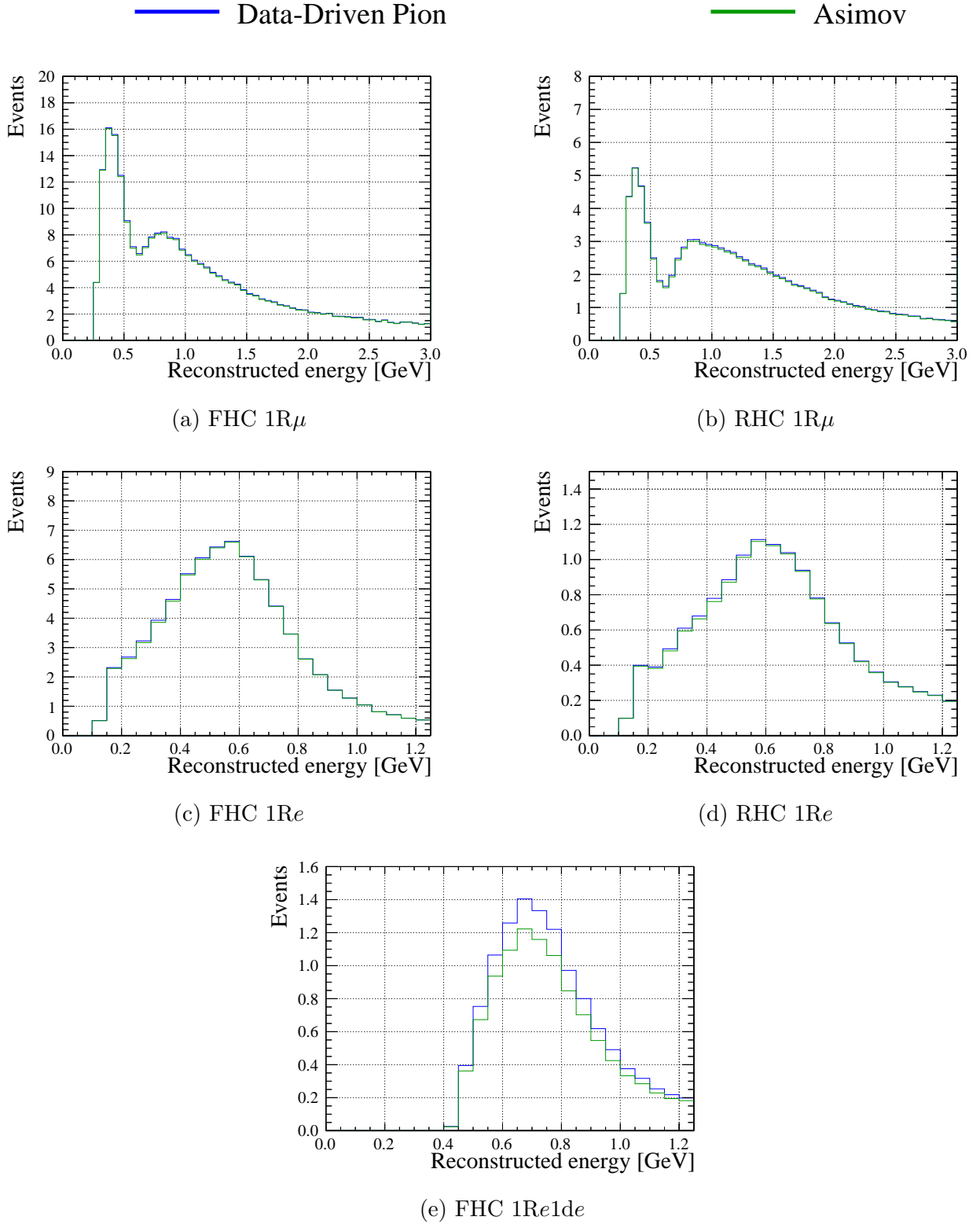
Figure 5.32: SK predictions for the data-driven pion kinematics simulated data set. The green line shows the nominal SK Asimov, with nominal BANFF Asimov best-fit systematic parameters. The blue line shows the SK prediction after applying the required weights to the nominal prediction - essentially, the SK simulated data set.
