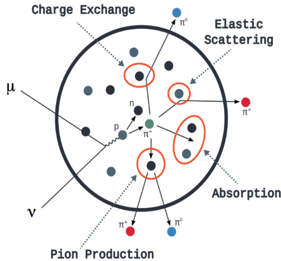
Figure 2.27: Schematic representation of different types of pion FSI. Taken from [99].
