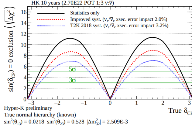
Figure 7.10: Sensitivity to exclude \sin\delta_{CP}=0 , using accelerator neutrinos, and assuming 10 years of Hyper-K data taking and normal hierarchy (known), as a function of the true value of \delta_{CP} . Three cases are compared: statistics only (i.e. no systematic errors) in solid black, the T2K 2018 level of systematic errors (dotted blue) and the improved HK error model (dashed red).
