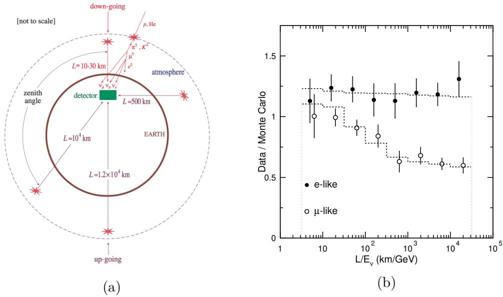
Figure 1.5: Illustration of Super-Kamiokande atmospheric neutrino detection technique (a) and ratio of data to Monte-Carlo prediction assuming no neutrino oscillations, for \nu_\mu and \nu_e atmospheric neutrino events seen by Super-Kamiokande (b). Figure from [41].
