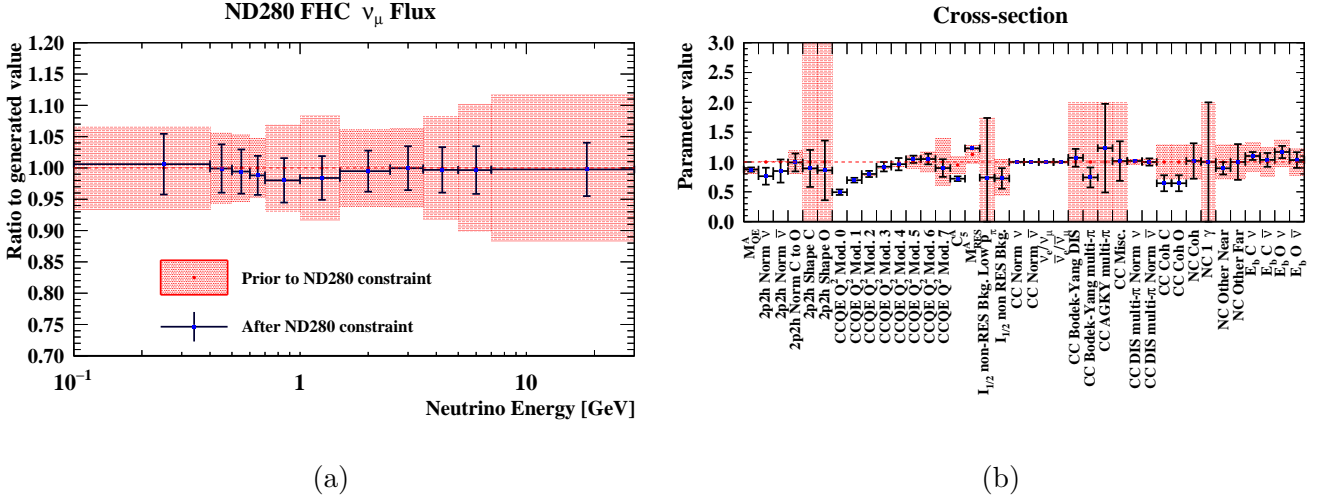
Figure 5.27: Flux (a) and cross-section (b) systematic parameters as a result of the near detector fit to the MINERνA pion suppression tune simulated data set. The red boxes show the nominal model prediction and errors.
