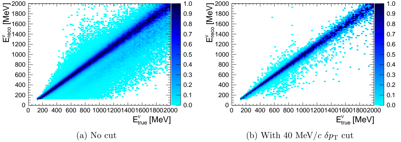
Figure 6.41: Reconstructed anti-neutrino energy ( E_{\text{reco}}^\nu ) as a function of true anti-neutrino energy ( E_{\text{true}}^\nu ), before (a) and after (b) the \delta p_T cut. The distributions are normalized column-wise to the largest entry per column.
