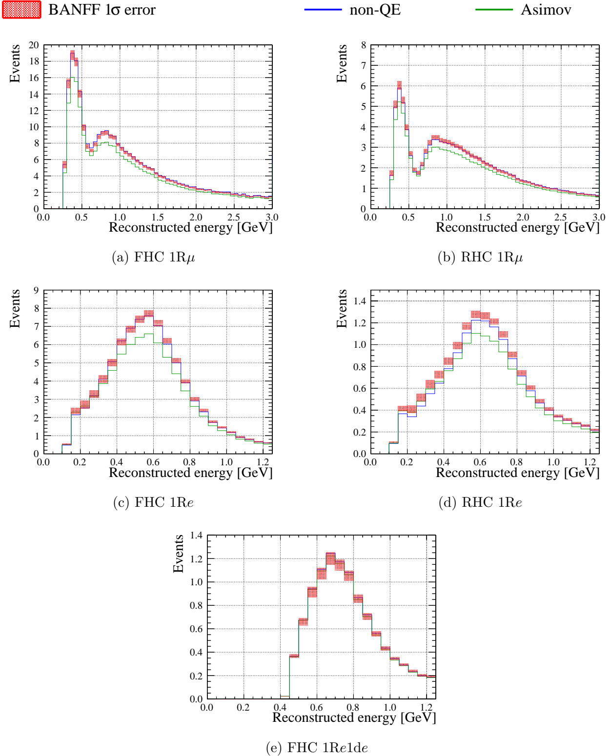
Figure 5.20: SK predictions for the CC0 \pi -focused simulated data set. The green line shows the nominal SK Asimov, with nominal BANFF Asimov best-fit systematic parameters. The blue line shows the SK prediction after applying the required weights to the nominal prediction - essentially, the SK simulated data set. The red shaded regions and their points show the errors and best-fit points from the BANFF fit to the simulated data set.
