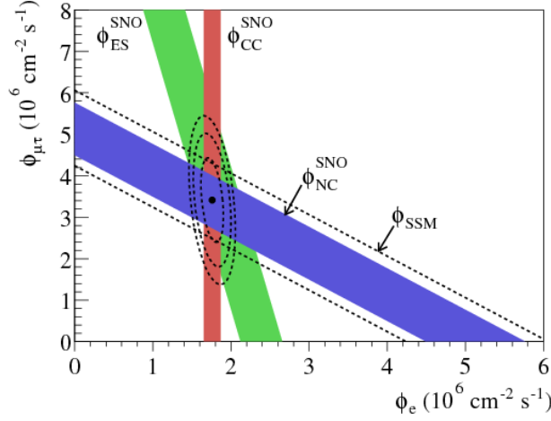
Figure 1.4: Solar neutrino flux in the three detection channels used in [34] - CC for charged current neutrino-nucleus interactions (sensitive to electron neutrino flux), NC for neutral current interactions (sensitive to the total neutrino flux) and ES for elastic scatters off electrons (sensitive to all neutrino flavors, but with an enhanced sensitivity to electron neutrinos). The dotted lines show the prediction of the Standard Solar Model. Figure from [34].
