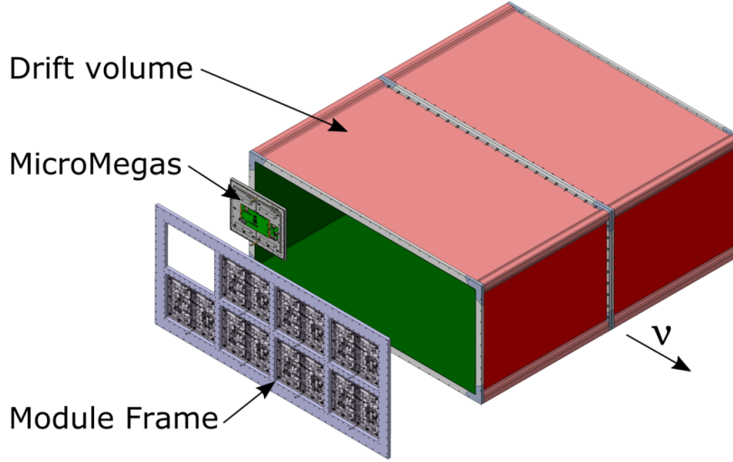
Figure 6.8: Schematic model of the HA-TPC.
