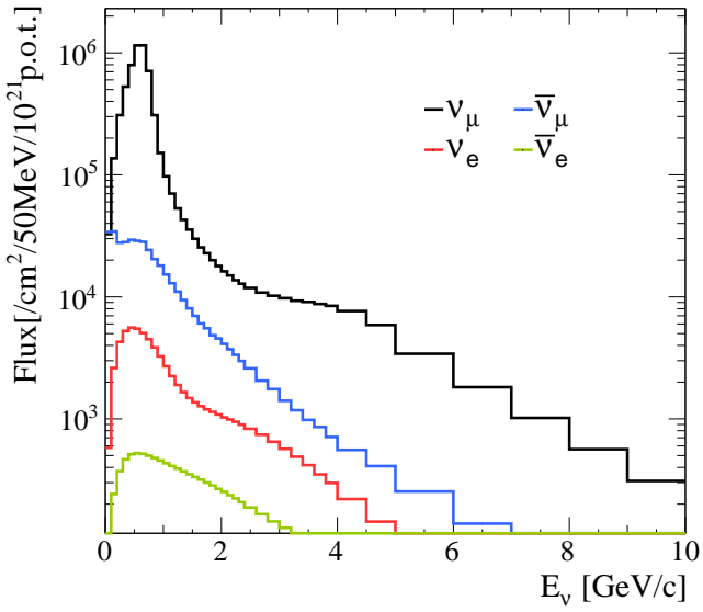
(c) Far Detector, Neutrino Mode
