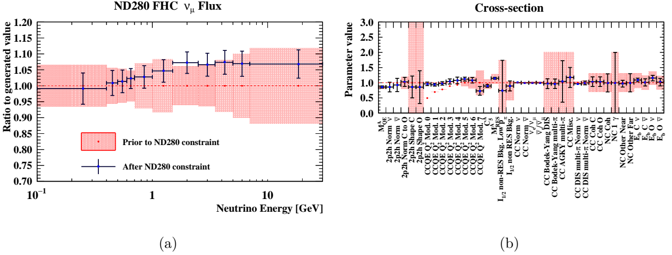
Figure 5.19: Flux (a) and cross-section (b) systematic parameters as a result of the near detector fit to the CC0 \pi -focused simulated data set. The red boxes show the nominal model prediction and errors.
