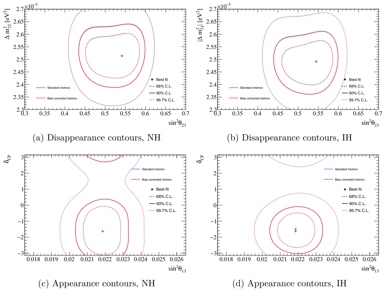
Figure 4.8: Comparison of bias-corrected Asimov fit results to the nominal Asimov results.
