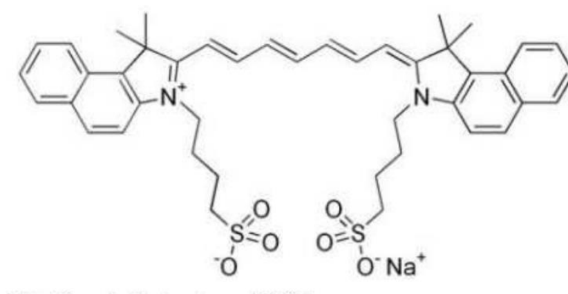
Figure 26: Molecular structure of Indocyanine Green (ICG). [239]
