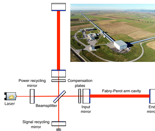
Fig. 1. Simplified optical layout of the advanced Virgo interferometer near Pisa in Italy. The configuration is a dual recycled Michelson with Fabry–Perot arm cavities. The GW signal imprinted in the phase of light is detected at the south port in this diagram. Inset: Aerial view of the detector, where one of the 3 km long arms is clearly visible. Credit: Virgo Collaboration.
