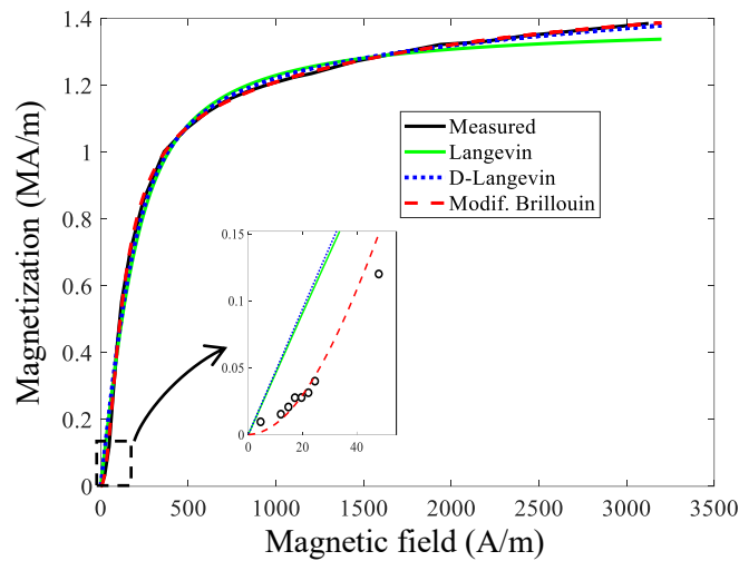
Fig. II.7 Modeled and measured magnetization curve without considering the stress effect for different anhysteretic functions for the grade M330-35A
