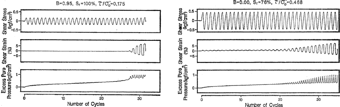
Figure 2.38 The behavior of soil under cyclic loading (Yoshimi 1989). a) full saturated sample b) unsaturated sample
