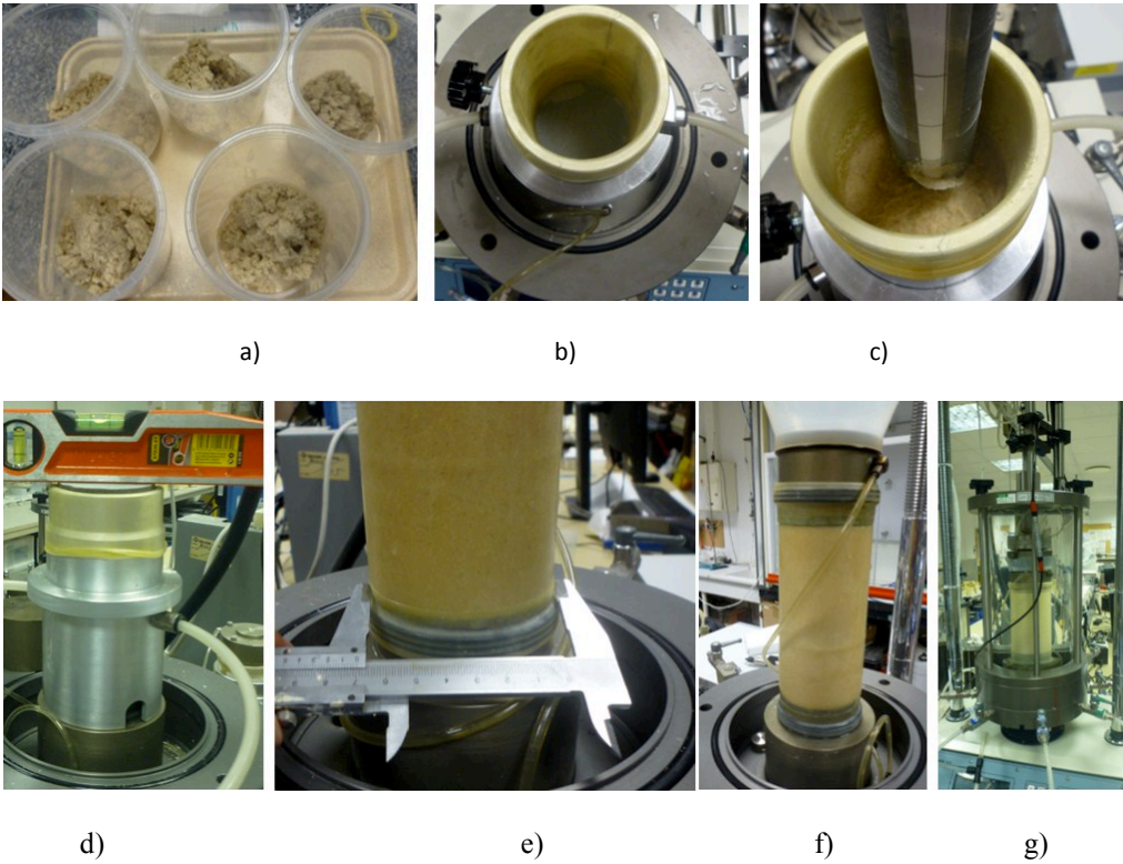
Figure 3.13 Sample preparation by wet tamping method
