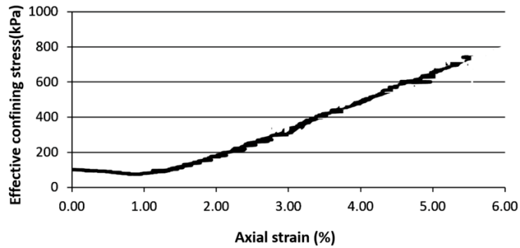
c) Effective confining stress versus axial strain
