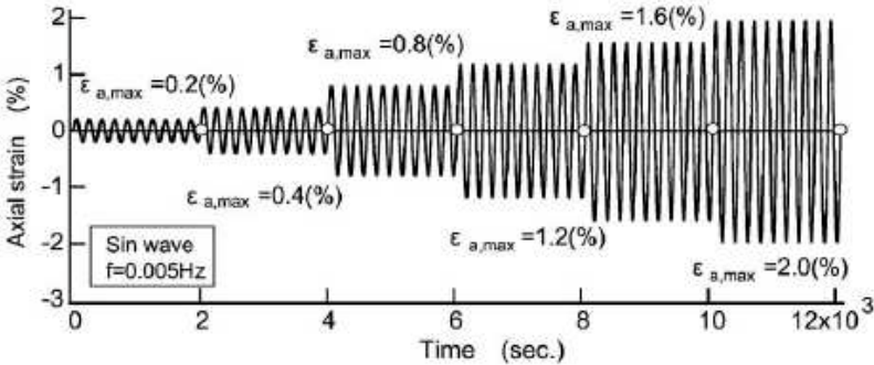
Figure 2.44 Time history of axial strain during cyclic loading process (Unno et al. 2008)
