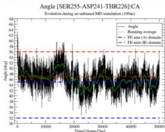
Figure 5. Evolution of the Ser255( C\alpha )–Asp241( C\alpha )–Thr226( C\alpha ) angle during an unbiased run (WT-MD). The angle time series from the WT-MD simulation is shown in black, and the angle running average (smoothing) is represented in green. The domains covering free energy (FE) wells A and B are represented by the dashed blue and red lines, respectively.
