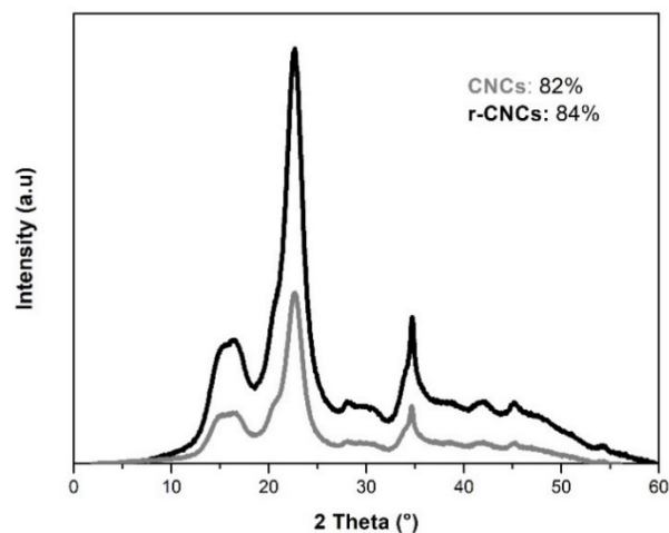
Figure 4.6 - XRD spectra of the CNCs and r-CNCs.
