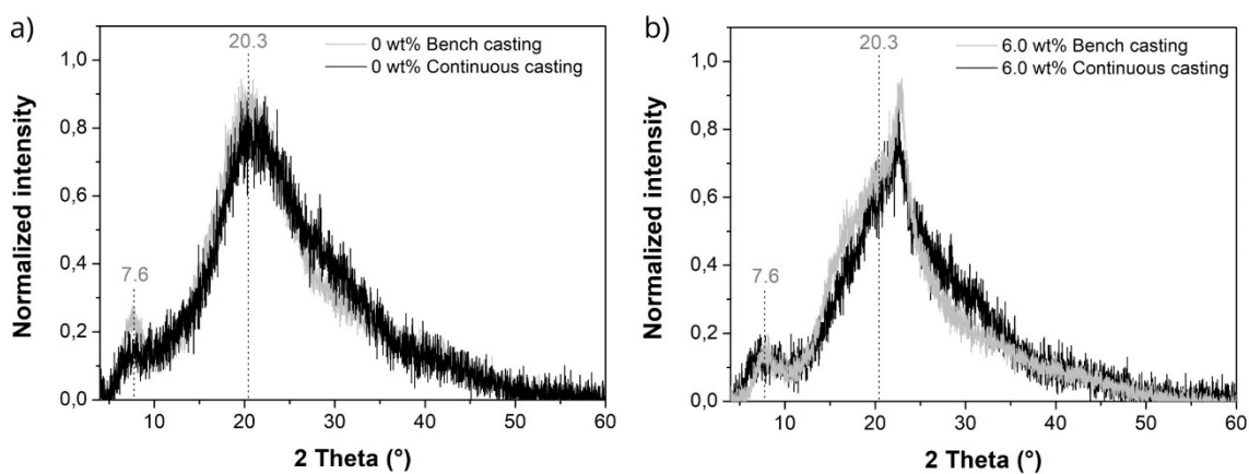
Figure 2.17 - XRD patterns of gelatin films with (a) 0 wt% CNCs and (b) 6.0 wt% CNCs obtained by bench and continuous casting.
