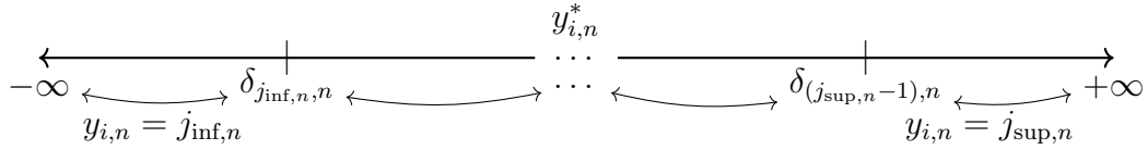
Figure 1.1 – Relation between latent variable and dependent variable
