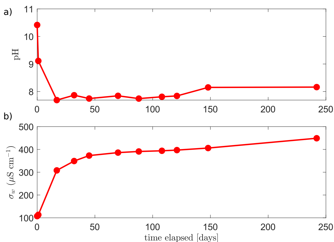
Figure 2.19: Example of the a) pH and b) water conductivity monitoring (after mixing) for the water-clay sample of red montmorillonite and initially de-ionized water.
