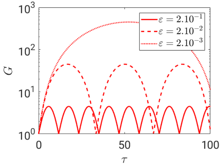
Figure 5.2: Energy gain G defined in (5.4) as a function of time \tau for the linearized problem around the stable point \mathbf{M}'_0 = (0, 0, 1)^T for \Sigma = 0.9 and \varepsilon = 2 \cdot 10^{-1} (continuous line), \varepsilon = 2 \cdot 10^{-2} (dashed line) and \varepsilon = 2 \cdot 10^{-3} (dotted line).
