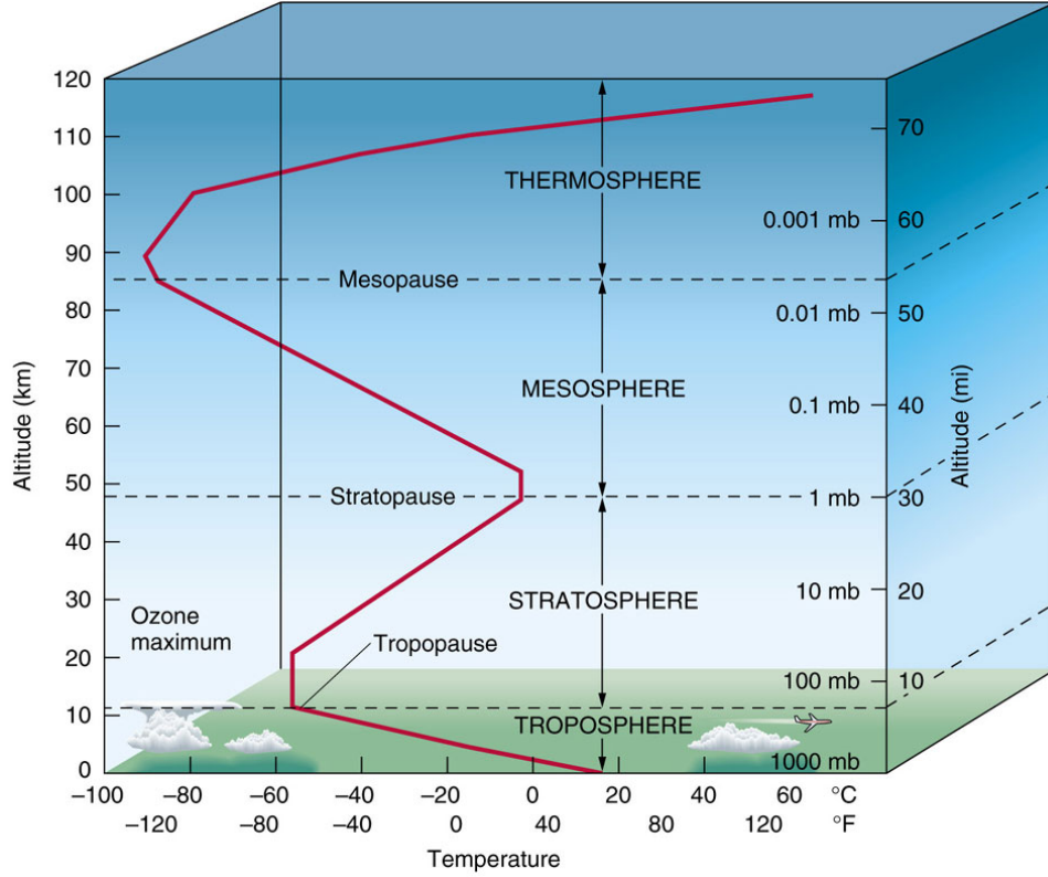
Figure 3.4: Vertical temperature profile of the atmosphere as a function of altitude. Source: University of Lagos (2012), http://unilaggeography2012.blogspot.com/p/gry-101-introduction-to-physical.html
