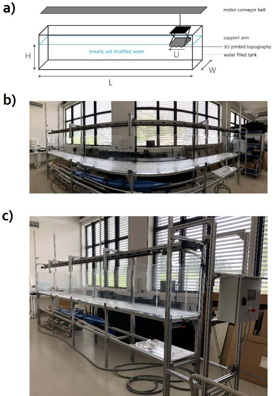
Figure 10.1: a) Schematics of the laboratory set up at LadHyX, similar to the one used by Aguilar et al. (2006), but with a larger tank, measuring L = 6 m long, W = 50 cm wide, filled by salty water of maximum height H = 50 cm, such that the buoyancy frequency equals N = 1.1 \text{ rad s}^{-1} . The topography mounted on an adjustable support arm can reach speed U up to 1 \text{ m s}^{-1} . b) Panoramic photo of the (empty) tank at LadHyX (sideview). c) Photo of the experimental setup from another perspective, showing the console piloting the motor conveyor belt placed at the top right end of the tank. The console controls the speed of the towed topography, and durations of the acceleration and deceleration phases.
