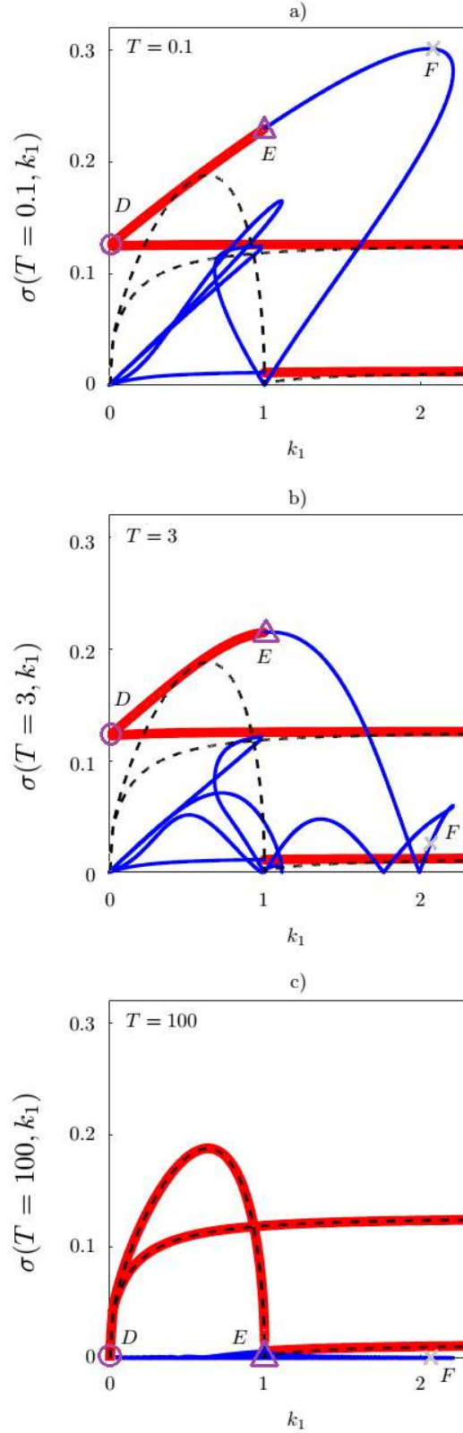
Figure 6.2: Plots of the optimal growth rate \sigma as a function of k_1 for T = 0.1 in a), T = 3 in b), and T = 100 in c), for stable and unstable resonant triads represented in thin blue and in bold red lines respectively. In c), \sigma has converged toward the growth rate \sigma_{\text{th}} of the classical triadic instability theory plotted as a dark dashed line on all the graphics. The points (E, D_-, D_+, F) from figure 6.1 are reported on all three figures, point D being in reality D_- , as D_- and D_+ lead to the same growth rate.
