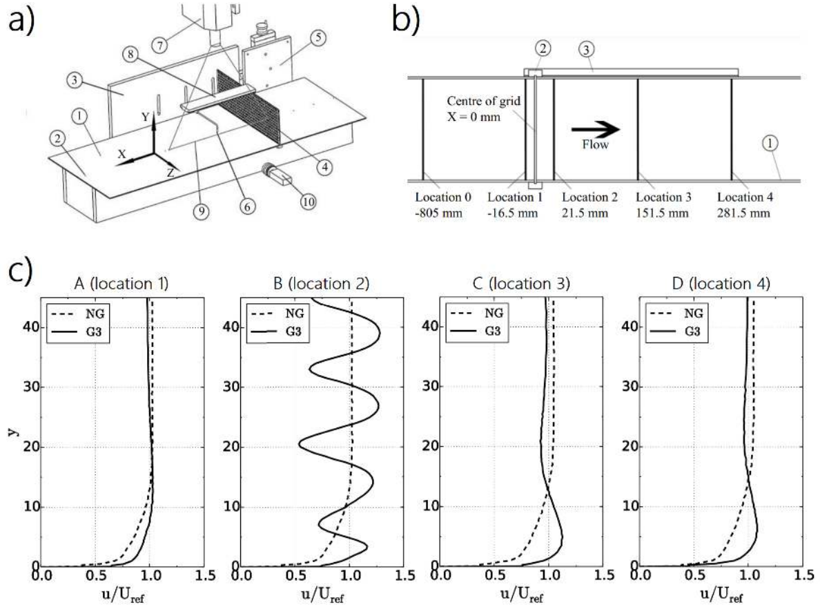
Figure 10.3: a) Experimental setup of Irps (2016) with a fixed surface lower wall in (1) where boundary layer flow is tracked. In (2), pressure tapings along the center line of the lower wall are used to measure pressure drops along the duct. (3) points out a background window with slots containing hot-wires, (4) is the grid around which pneumatic probe traverses in the wall normal direction ( Y axis) at five selected locations defined on figure b). A linear actuator mechanism for traversing the probe is fixed on the outside of the wind-tunnel (5). Non-intrusive PIV setup is used for visualising the horizontal velocity field u in the intended measuring area (9) and is composed of a non-reflective glass (8), a laser head (7), a the camera (10). b) View of the tunnel from above defining five locations. c) Horizontal velocity profile for a grid G3 of 9 mm holes, 3 mm strut, with a porosity 0.563 and a pressure drop factor 2.27, at the four locations 1, 2, 3 and 4, corresponding to the plots A, B, C and D respectively, U_{ref} being a referenced velocity. Dashed curves correspond to the absence of grid, and the continuous curves to the presence of grid G3. From Irps (2016).
