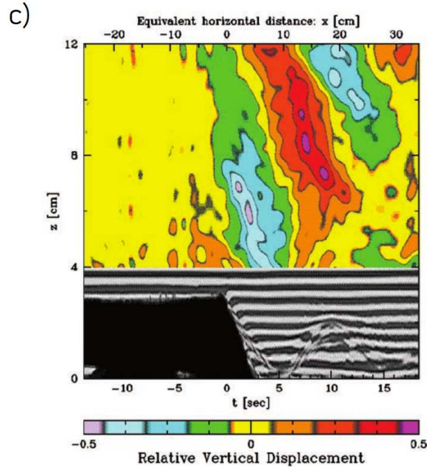
Figure 2.2: a) Schematic of Sutherland's experiment showing the tank in which the step-shaped topography of height 2H is towed at a constant speed U in a linearly stratified fluid. b) Synthetic schlieren uses a digital camera to capture the image of horizontal lines after the light source. c) Time series of the relative vertical displacement z as a function of time t . The image of the towed topography is superimposed below z = 4 cm keeping the same coordinates z , but as a function of the horizontal coordinates x = Ut , the whole picture c) being upside down compared to a). From Sutherland (2002).
