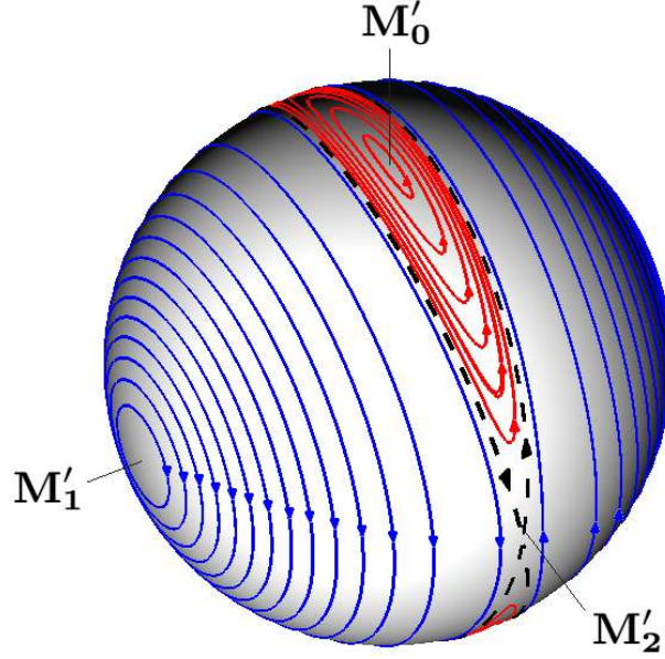
Figure 5.1: Trajectories on the sphere unit \mathcal{E} = 1 in the (M'_0, M'_1, M'_2) space with J_2 = (1 - \varepsilon)J_0 , \varepsilon = 2 \cdot 10^{-2} , J_1 = (1 - \Sigma)J_0 and \Sigma = 0.9 . The point \mathbf{M}'_1 = (0, 1, 0)^T is stable and close trajectories around \mathbf{M}'_1 are plotted in blue, \mathbf{M}'_0 = (0, 0, 1)^T is stable too and close trajectories around \mathbf{M}'_0 are in red.
