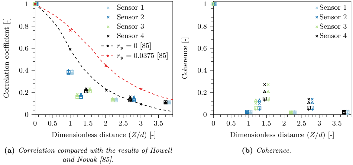
Figure 5.11: Coherence and correlation at different amplitudes but the same dimensionless speed ( \omega_q = 1.14 ). The amplitudes are \times = 0.059 , \Delta = 0.041 , \square = 0.0062 and + = 0.0028.
