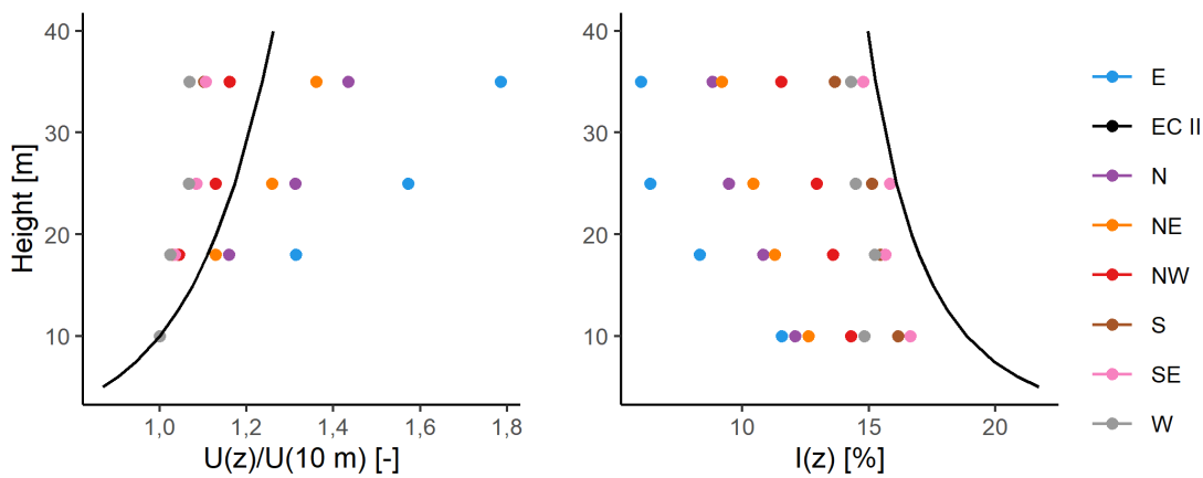
Figure 4 Mean incoming speed and turbulence profiles (filled dots) compared with the Eurocode profile for terrain category II (solid lines).
