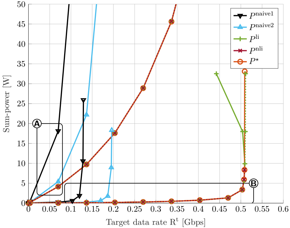
Figure 6.4: Sum-power vs. target data rate R_{b,m}^t = R^t with G_{\text{amp}} \in \{-10, 10\} dB (respectively A and B), and 0.1 FS per 100 km 2 .
