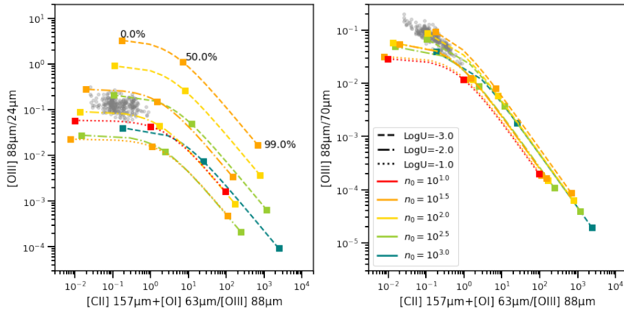
FIGURE B.1: Representation of the data of the region 30 Doradus and models with constant pressure for [\text{O III}] 88\mu\text{m}/\text{MIPS } 24\mu\text{m} as a function of ([\text{C II}]+[\text{O I}])/[\text{O III}] (left panel), and [\text{O III}] 88\mu\text{m}/\text{MIPS } 70\mu\text{m} as a function of ([\text{C II}]+[\text{O I}])/[\text{O III}] (right panel). Each model is represented with a color for the initial density and a line style for the ionization parameter, and the lines are following the proportion of PDR emission, with the markers representing the proportions of 0%, 50 % and 99%. The models displayed are calculated for an age of star forming burst of 4 Myrs, and only the data from the 30 Doradus region are represented.
