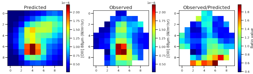
FIGURE 4.11: Similar to Figure 4.6, but for N158.
