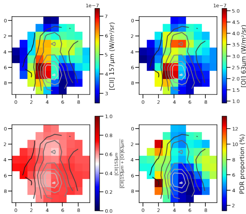
FIGURE 4.39: Similar to Figure 4.35, for the region N158.
