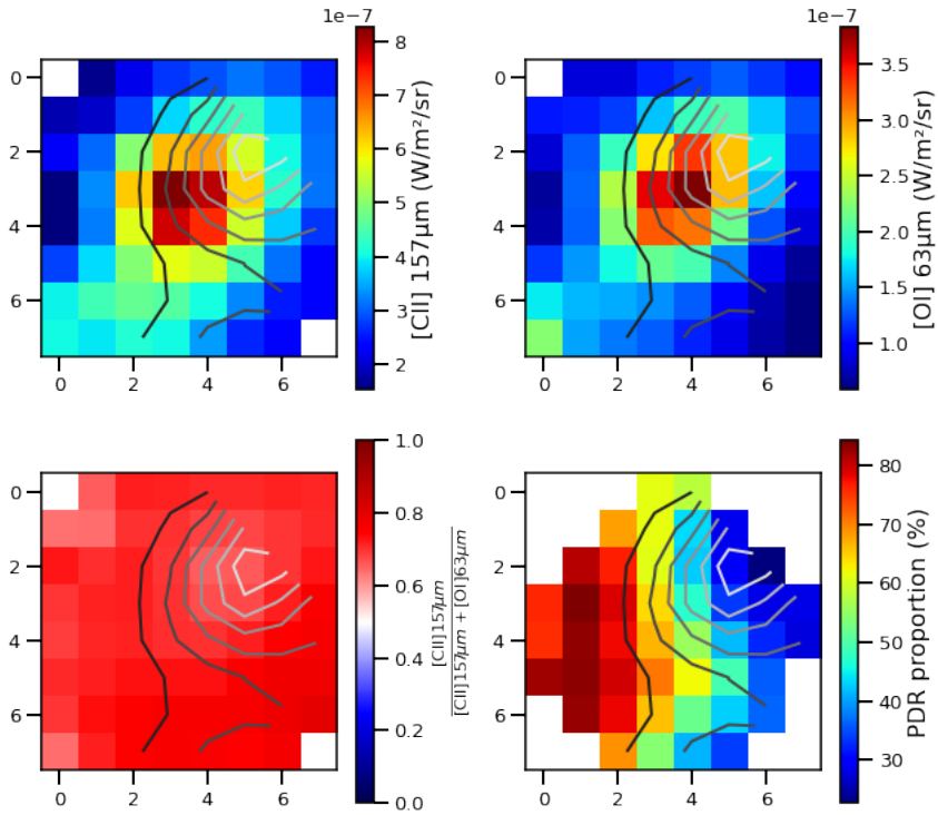
FIGURE 4.42: Similar to Figure 4.35, for the region N44.
