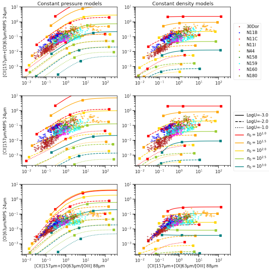
FIGURE 5.8: The ratio of ([C\ II] + [O\ I]) / 24\mu\text{m} as a function of the ratio we use to disentangle the PDR emission from the ionized region emission, namely ([C\ II] + [O\ I]) / [O\ III] (upper panels), and the ratio of each cooling line over MIPS 24\mu\text{m} separately, in middle and lower panel. On the left panels, data are superimposed with the constant pressure models, and on the right panel with constant density models. Models are represented with different proportions of PDR along each line, with the markers to indicate some specific values: 0%, 50% and 99% from lower to higher values of ([C\ II] + [O\ I]) / [O\ III] . The line colors designate different densities and the line types different \log(U) , all described in the legend to the right of the plots.
