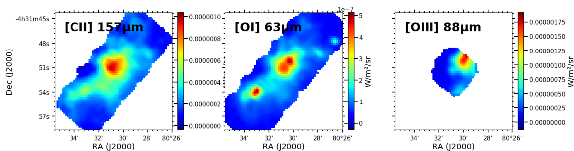
FIGURE 2.20: Similar to Figure 2.4, for the region N44.
