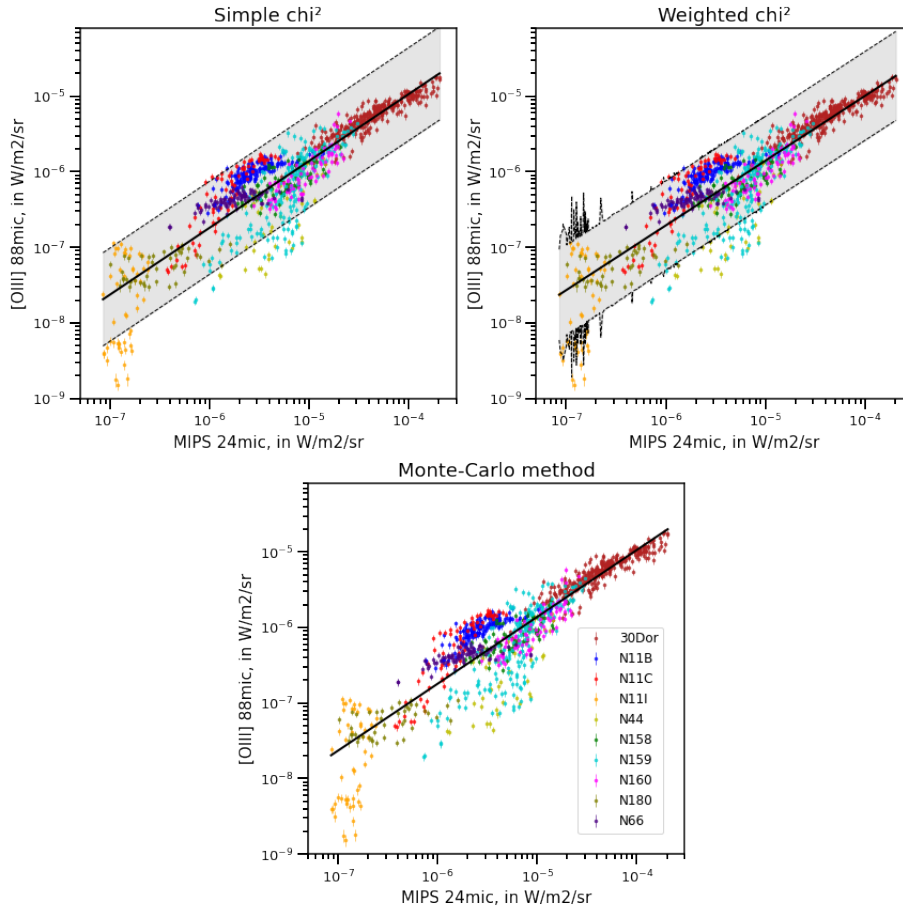
FIGURE A.1: Linear fits between [O III] 88\mu m and 24\mu m for the three methods. The 95% confidence intervals are represented with dashed lines and grey fillings for the simple and weighted \chi^2 methods. The confidence interval is not determined for the Monte-Carlo method. The upper right panel, corresponding to the weighted \chi^2 , is identical to the Figure 4.1 in Chapter 4, showing the fit of the correlation.
