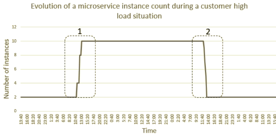
FIGURE 4.4: Microservices auto-scaling based on message-bus metrics (Screenshot from our grafana dashboard)
