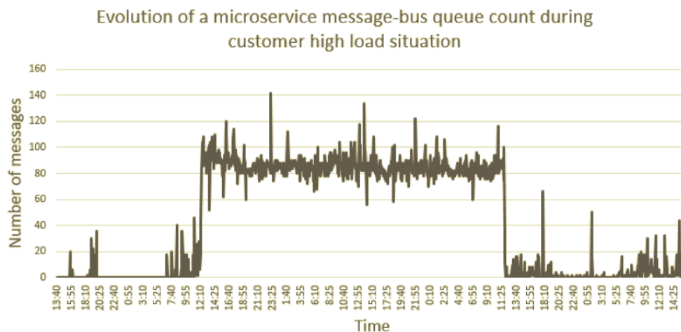
FIGURE 4.5: Increase in incoming message during the scaling event in Figure 4.4
