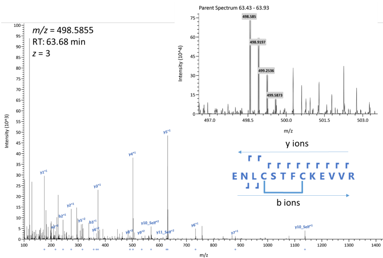
Figure 5: MS/MS spectrum of the intra chain LAN cross-link between two cysteines in the peptide sequence. This peptide sequence was found in \alpha_{s2} casein of the Qishta protein. Amino acids are referred with their abbreviation code.
