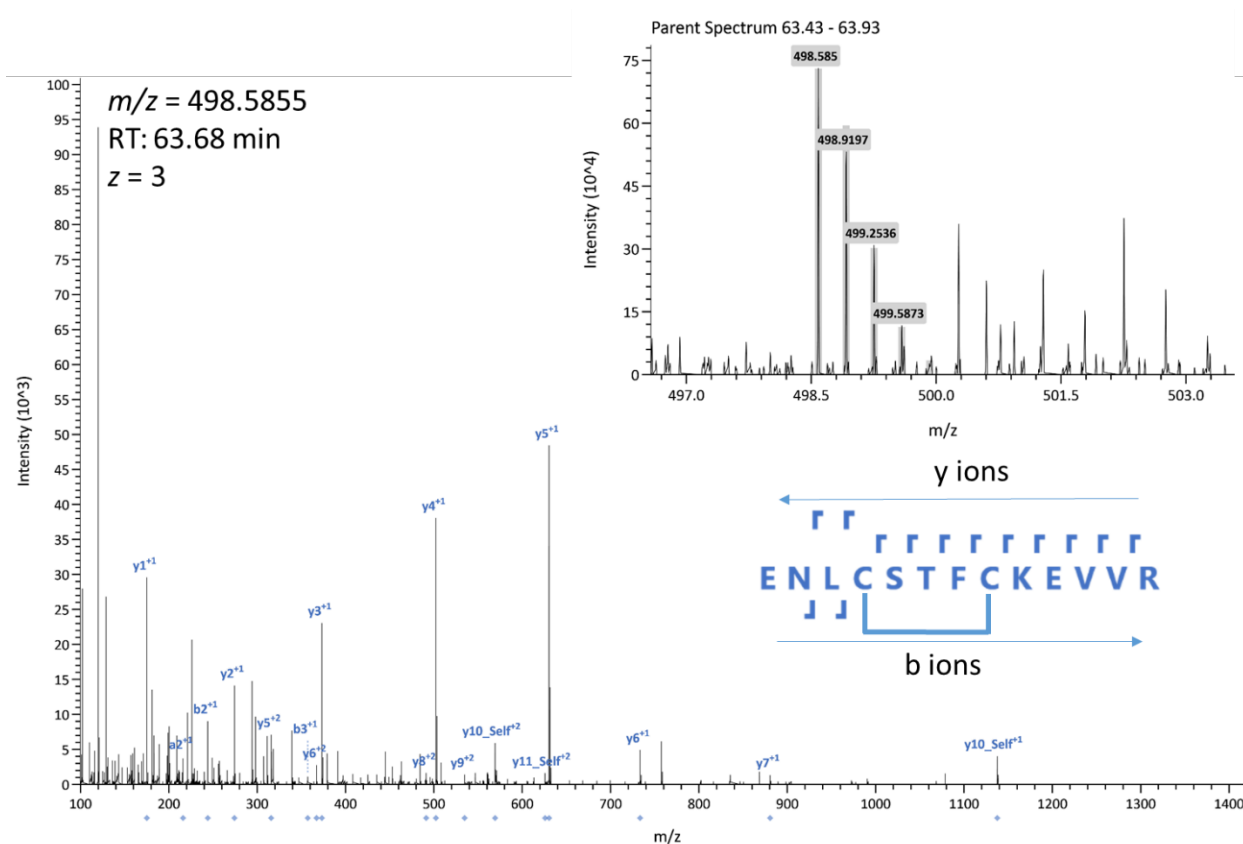
Figure 5: MS/MS spectrum of the intra chain LAN cross-link between two cysteines in the peptide sequence. This peptide sequence was found in \alpha s2 casein of the Qishta protein. Amino acids are referred with their abbreviation code.
