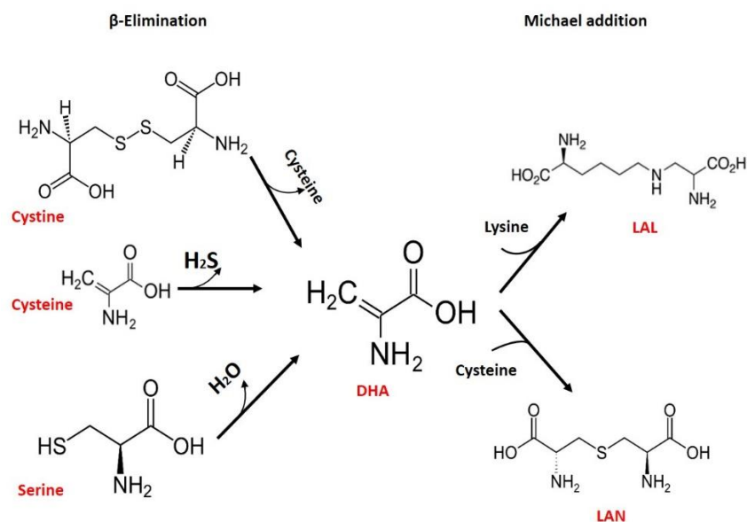
Figure 3: The mechanism of LAL and LAN formation. β-elimination of cystine, cysteine or serine resulting from dehydroalanine formation. Michael addition of lysine or cysteine yielding LAL or LAN respectively.
