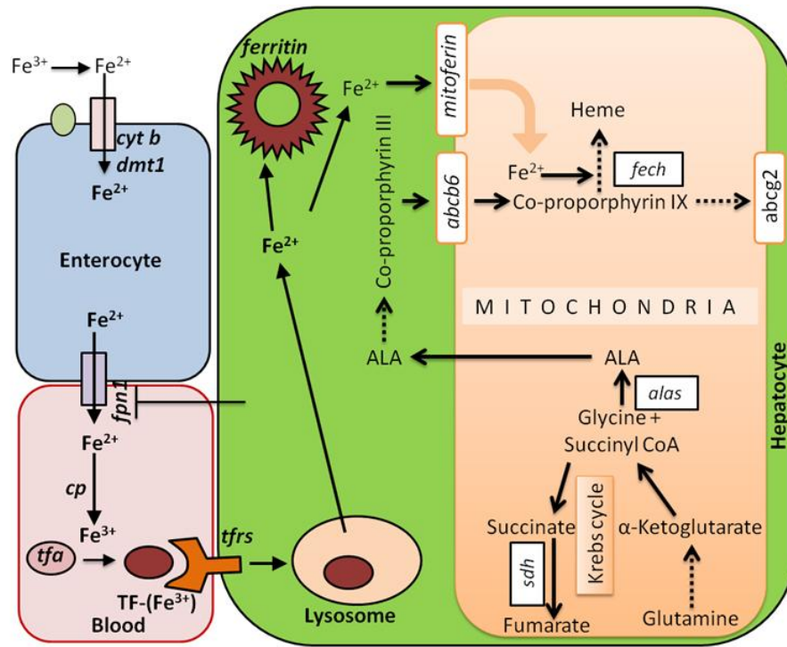
Figure 13: Iron/heme homeostasis
