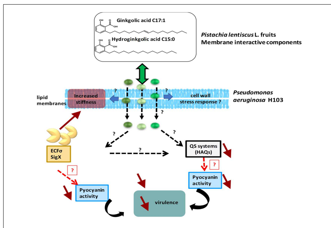
Figure 20. Putative mode of action of ginkgolic acids from Pistachia lentiscus on P. aeruginosa H103.
