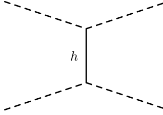
Figure 1.8: The z, w^+ \rightarrow z, w^+ scattering mediated by h .
