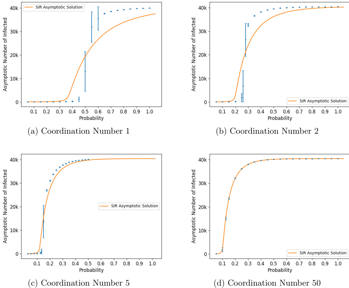
Figure 6.3: Evolution of the final number of infected cases as a function of the infection probability for different coordination radii r , compared to the asymptotic solution of the SIR model. The optimal factor found for the cases (a),(b),(c) and (d) are respectively: \rho = 0.27, 0.42, 0.50, 0.99 .
