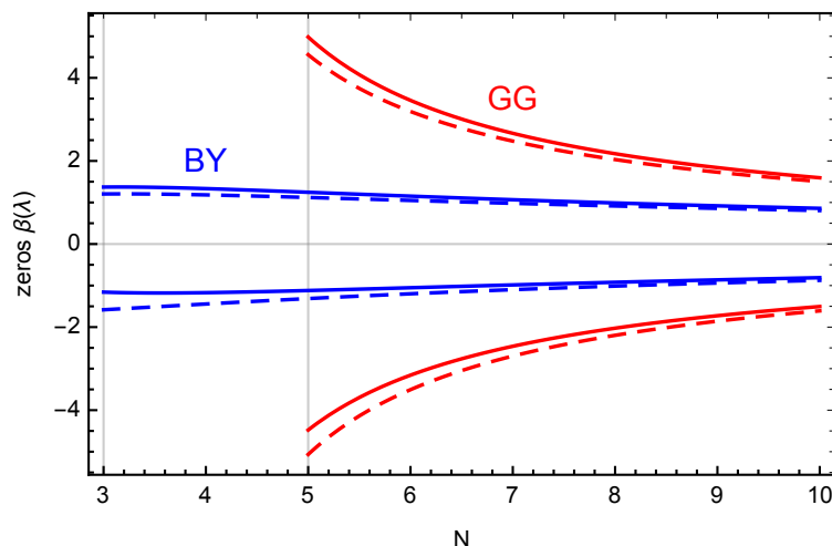
Figure 4.4: Zeros of \beta(\lambda) as a function of N for BY (blue) and GG (red) models. The solid lines correspond to y = y_{\text{UV}} = 0 , while the dashed ones to y = y_{\text{IR}} . The numerical values correspond to n_g = 10N , however other choices can be easily inferred knowing that the zeros scale as \lambda^* \sim n_g^{-1} .
