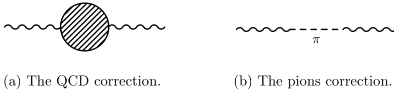
Figure 1.11: The total propagator's correction (left) and specifically the pions correction (right).
