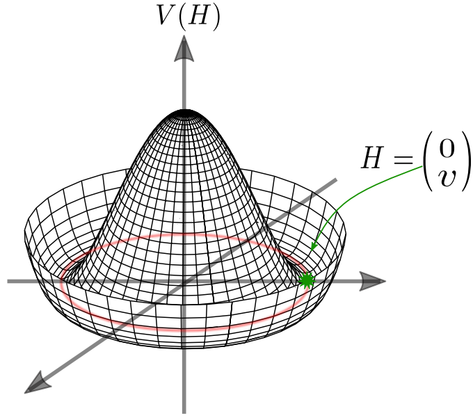
Figure 1.9: Sketch of the Higgs Potential, often called "Mexican Hat". The possible vacua are highlighted in red, and the chosen ground state has been positioned in green.
