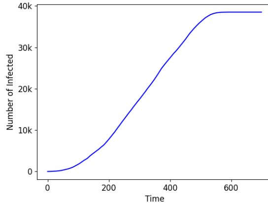
Figure 6.2: Evolution of the number of Infected, in a Lattice of size 200 \times 200 . The value of \gamma and \epsilon have been respectively fixed to 0.7 and 0.1
