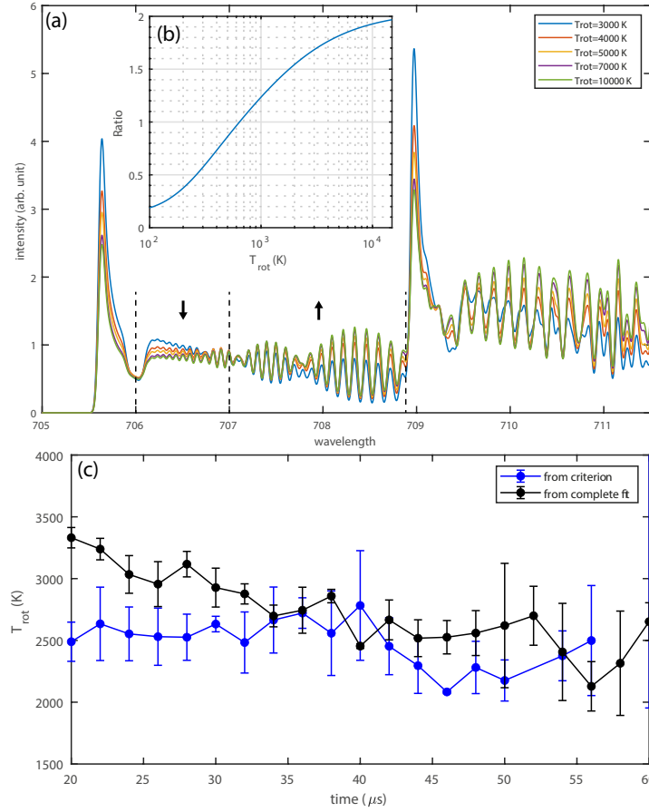
Figure 4.18: (a) Example of TiO spectrum ( \Delta v = 0 ) calculated for various T_{\text{rot}} (b) ratio of the integrated spectrum C_{\text{TiO}} = \int_{707}^{708.9} I / \int_{706}^{707} I depending on the temperature. (c) Comparison of the calculated T_{\text{rot}} from the ratio of the integrated spectrum and from a complete fit.
