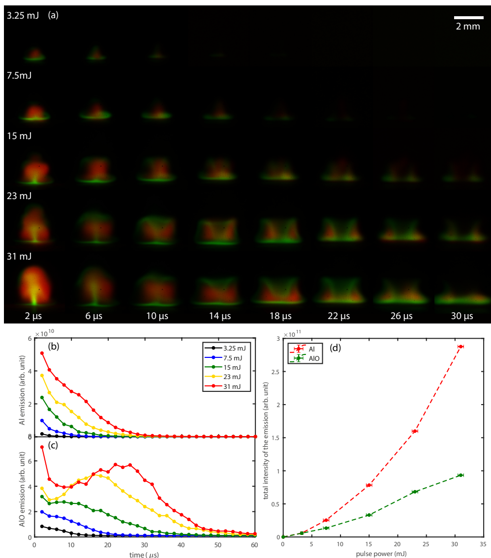
Figure 4.15: (a) dynamics of the plasma observed in false color at different delays after the ablation of an aluminum oxide target in air. Aluminum emission is in red and AlO( B^2\Sigma^+ ) emission is in green. (b) Intensity of the Al(I) emission integrated on the whole image. (c) Intensity of the AlO( B^2\Sigma^+ ) emission integrated on the whole image. (d) Intensities of the Al and AlO emission integrated on the whole image and time.
