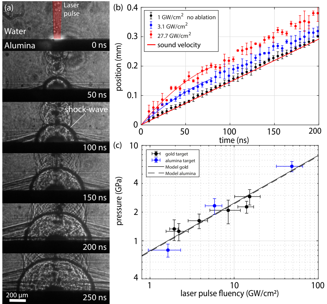
Figure D.2: (a) Shadowgraph images of the ablation of an alumina target in water for the different delays. (b) Time evolution of the shock wave position averaged on 4 measurement on gold target at different fluency. The red line correspond to the propagation of a wave at the sound velocity in water (1483 m/s). The black solid curves represents the second order polynomial fit on the data form time below 60 ns. These fit are used to determine the initial velocity of the shock-wave. (c) Measured pressure on gold target and alumina target using the initial velocity of the shock-wave for different fluency of the laser. The black solid line corresponds to the Berth-Fabbro Model.
