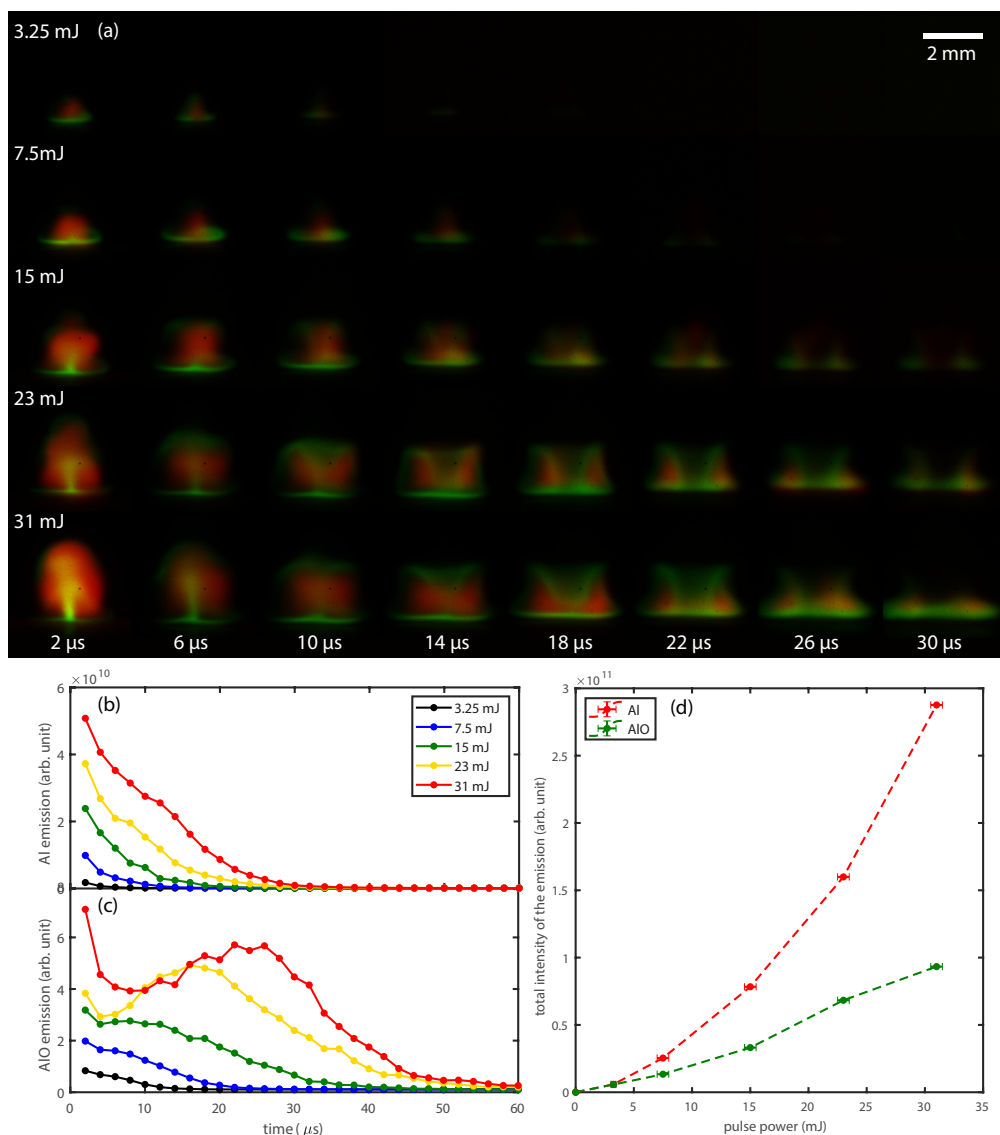
Figure 4.15: (a) dynamics of the plasma observed in false color at different delays after the ablation of an aluminum oxide target in air. Aluminum emission is in red and \text{AlO}(\text{B}^2\Sigma^+) emission is in green. (b) Intensity of the \text{Al}(\text{I}) emission integrated on the whole image. (c) Intensity of the \text{AlO}(\text{B}^2\Sigma^+) emission integrated on the whole image. (d) Intensities of the Al and AlO emission integrated on the whole image and time.
