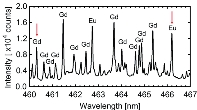
Fig. 7 LIBS spectroscopy. Typical atomic emission observed on a sample of Gd 2 O 3 :Eu nanoparticles. The red arrows show both lines used to quantify the atomic ratio [Eu]/[Gd].
