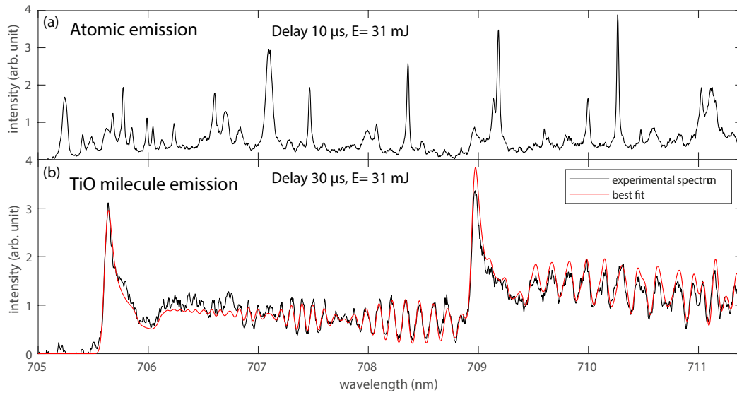
Figure 4.20: (a) TiO spectrum for a delay of 10\ \mu\text{s} dominated by atomic emission. (b) Example of TiO spectra in black (lateral position 0 mm, height 0 mm, delay 30\ \mu\text{s} , pulse energy 31 mJ) and corresponding best fit in red.
