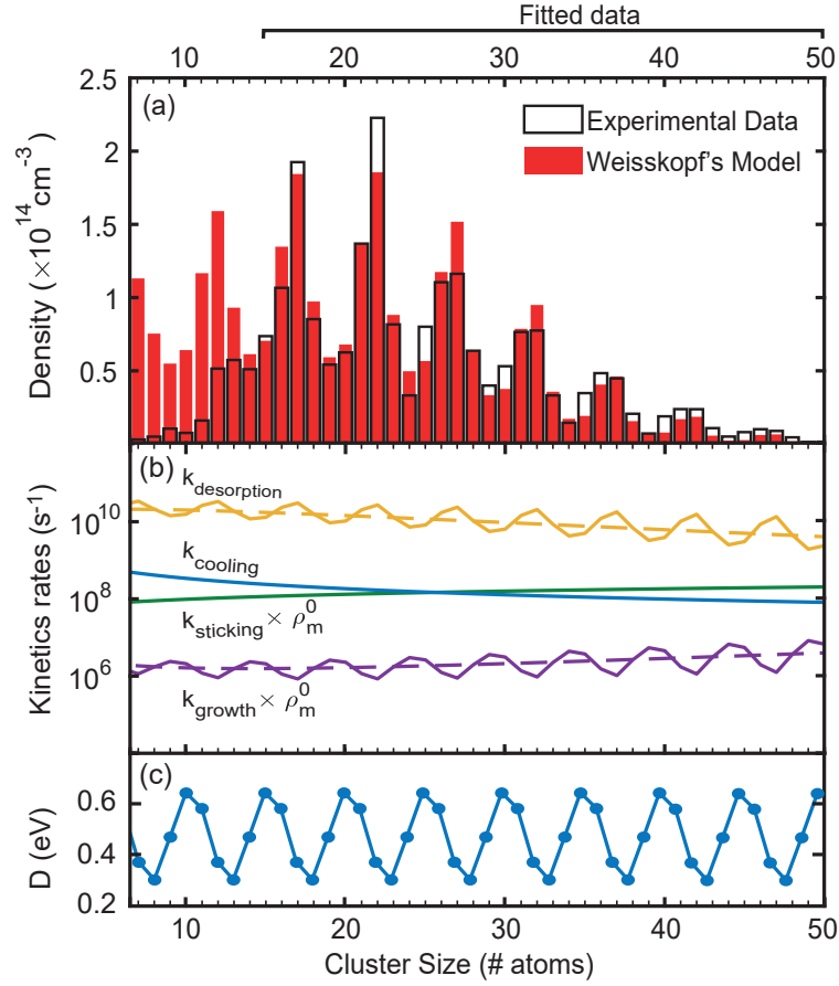
Figure 2.11: (a) Experimental distribution obtained for \rho_{\text{He}} = 6 \pm 0.6 \times 10^{19} \text{ cm}^{-3} (black) and calculated distribution (red) at the same helium density given the fitted parameters table. The cluster size corresponds to the total number of atoms in each identified cluster, whatever the cluster stoichiometry. (b) Cooling rates, desorption rates, sticking, and growth rate for the initial monomer concentration and the parameters of table 2.5. Dashed lines correspond to a constant value of D , while solid lines correspond to D modulated by a sine as shown in (c) and leading to the observed magic number features.
