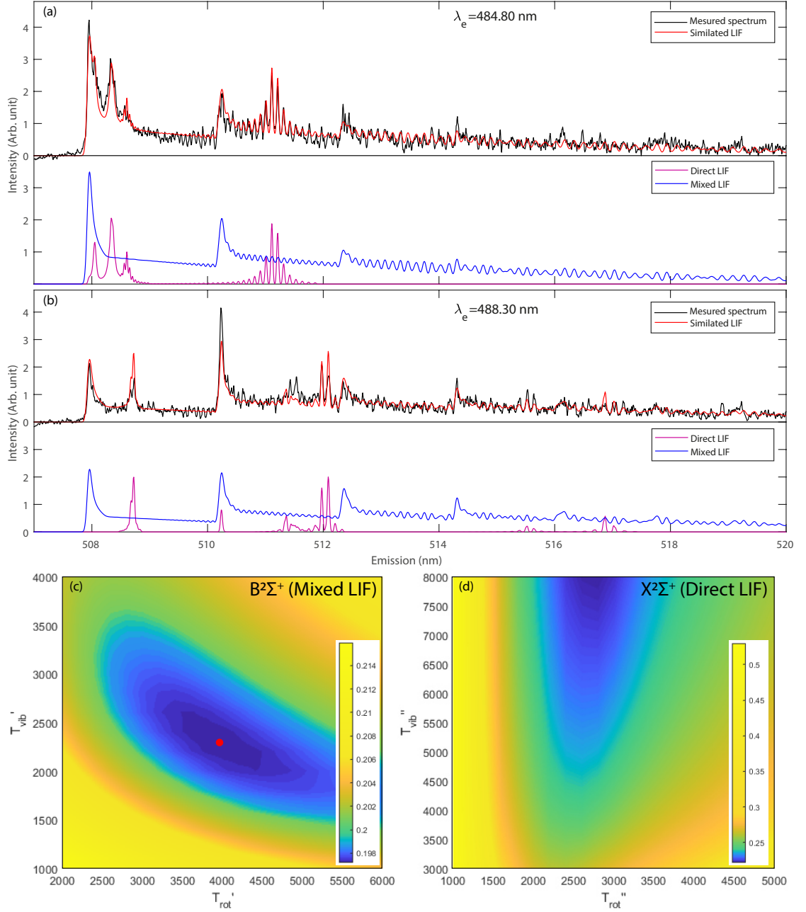
Figure 5.7: Example of fitted LIF spectrum (red) on measured spectrum for a delay of 30 \mu s (black) for the excitation wavelength 484.80 nm (a) and 488.30 nm (b) considering a single temperature T_{X^2\Sigma^+} for the ground state. Lower panels represent the relaxed LIF contribution (blue) and the direct LIF contribution (magenta). (c) corresponds to the residues map of (b) depending on T'_{rot} and T'_{vib} describing the excited relaxed state for the other parameters kept constant. The red point corresponds to the fitted parameters. (d) corresponds to the residues map of (b) depending on T''_{rot} and T''_{vib} describing the ground state for the other parameters kept constant. In the following fit, T''_{rot} = T''_{vib} = T_{X^2\Sigma^+} in order to avoid the T''_{vib} diverging.
