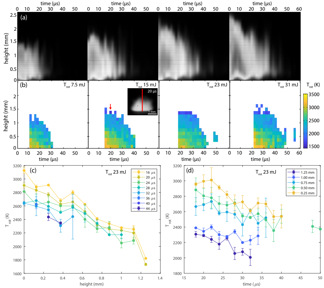
Figure 4.26: (a) Plasma emission for TiO emission range in the center vertical axis. (b) T_{\text{rot}} measured on the vertical center of the plasma. (c) and (d) rotational temperatures for the 23 mJ pulse depending on the height and delay time.
