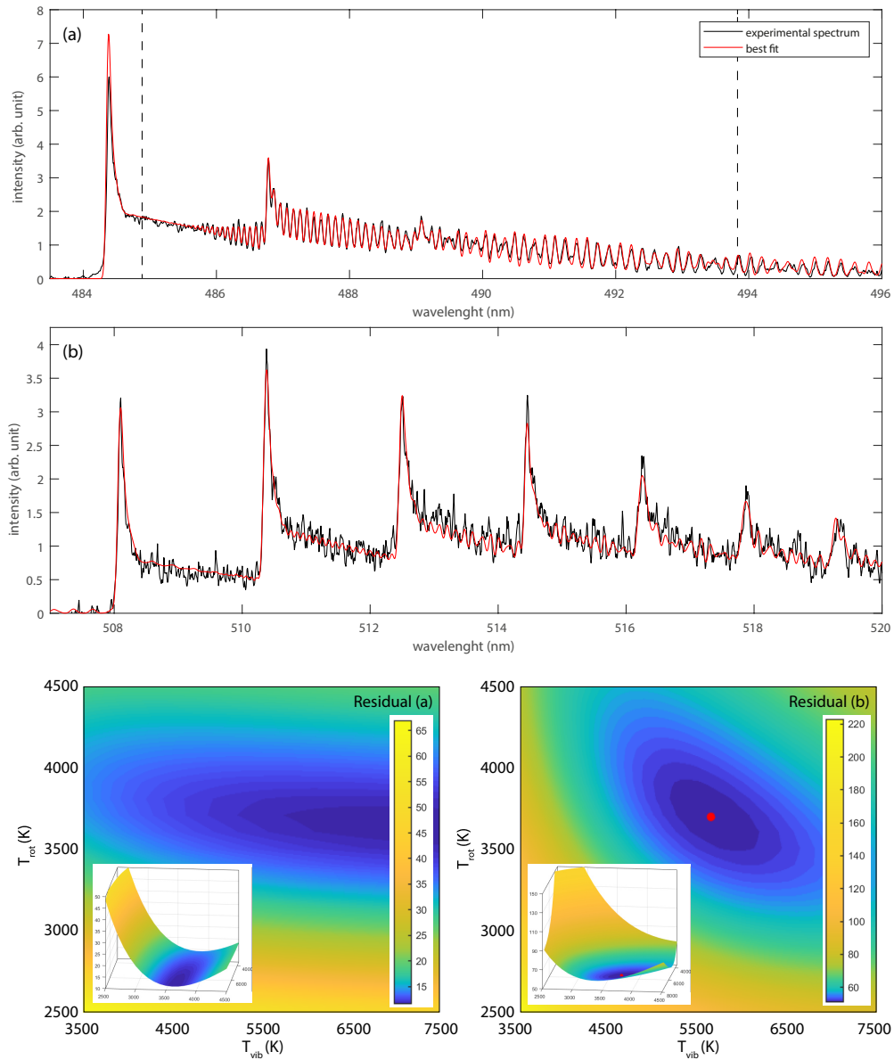
Figure 4.19: Example of AIO spectra (lateral position 0 mm, height 0 mm, delay 10 \mu s, pulse energy 24.5 mJ) for \Delta v = 0 (a) and \Delta v = -1 (b). Red curves correspond to the calculated spectra determined according to the fitting process described in the main text and correspond to T_{rot} = 3693 K and T_{vib} = 5644 K. Dashed lines in (a) delimit the fitting region. Below are plotted the residual maps depending on the temperatures. Other fitting parameters are kept constant. Red dots represent the fit convergence.
