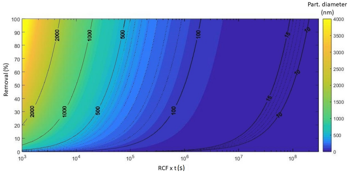
Figure 3: Percentage of removal for different size of \text{Gd}_2\text{O}_3 particles (density 7.41 \text{ g.cm}^{-3} ) in water as a function of the Relative Centrifugal Force times the centrifugation duration. The tube filling height is 7 cm. The velocity of sedimentation is based on the Stoke's law. The sub-micronic particles selection performed corresponds to \text{RCF} \times t = 50 * 600 = 3 \times 10^4 .
