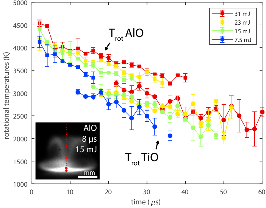
Figure 4.28: Comparison of the rotational temperatures of AlO and TiO molecules depending on delay time for different pulse energy. The temperatures are averaged on the two closest fibers to the target on the central axis of the plasma as represented in the inset.
