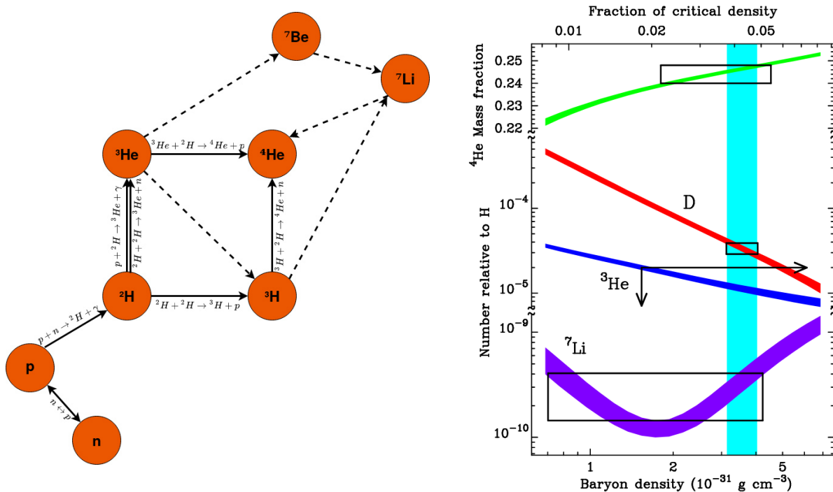
Figure 1.7 – Left panel: diagram of the Big-Bang nucleosynthesis with the main reactions. Right panel: predicted abundances of the light nuclei from the Big-Bang nucleosynthesis from [33].
